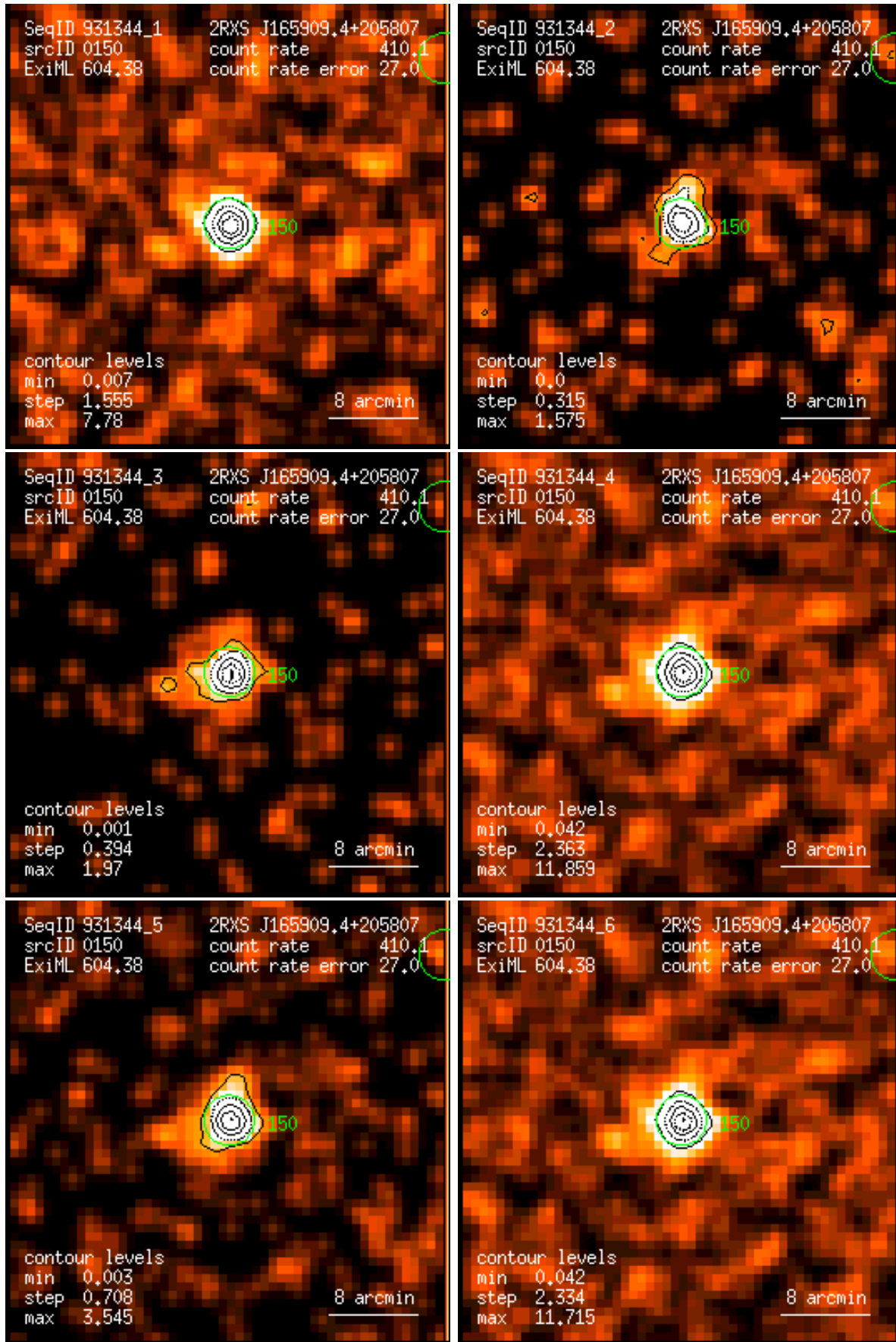
Figure 150: RASS 931344: detection 0150: band rate images, Gaussian filter: (1) PSPC channels 11 – 41, (2) 52 – 90, (3) 91 – 201, (4) 11 – 235, (5) 52 – 201, (6) 11 – 201. Broad band rates in counts/ks. Band rate contour levels in counts/ks/arcmin 2 .
