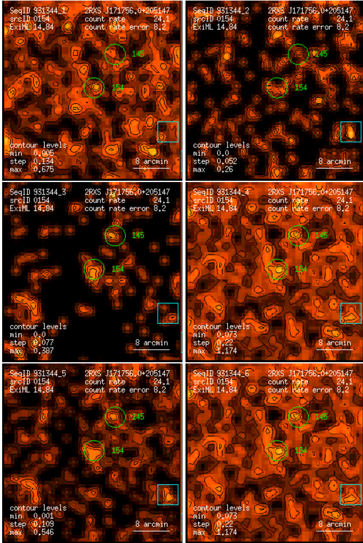
Figure 154: RASS 931344: detection 0154: band rate images, Gaussian filter: (1) PSPC channels 11 – 41, (2) 52 – 90, (3) 91 – 201, (4) 11 – 235, (5) 52 – 201, (6) 11 – 201. Broad band rates in counts/ks. Band rate contour levels in counts/ks/arcmin 2 .
