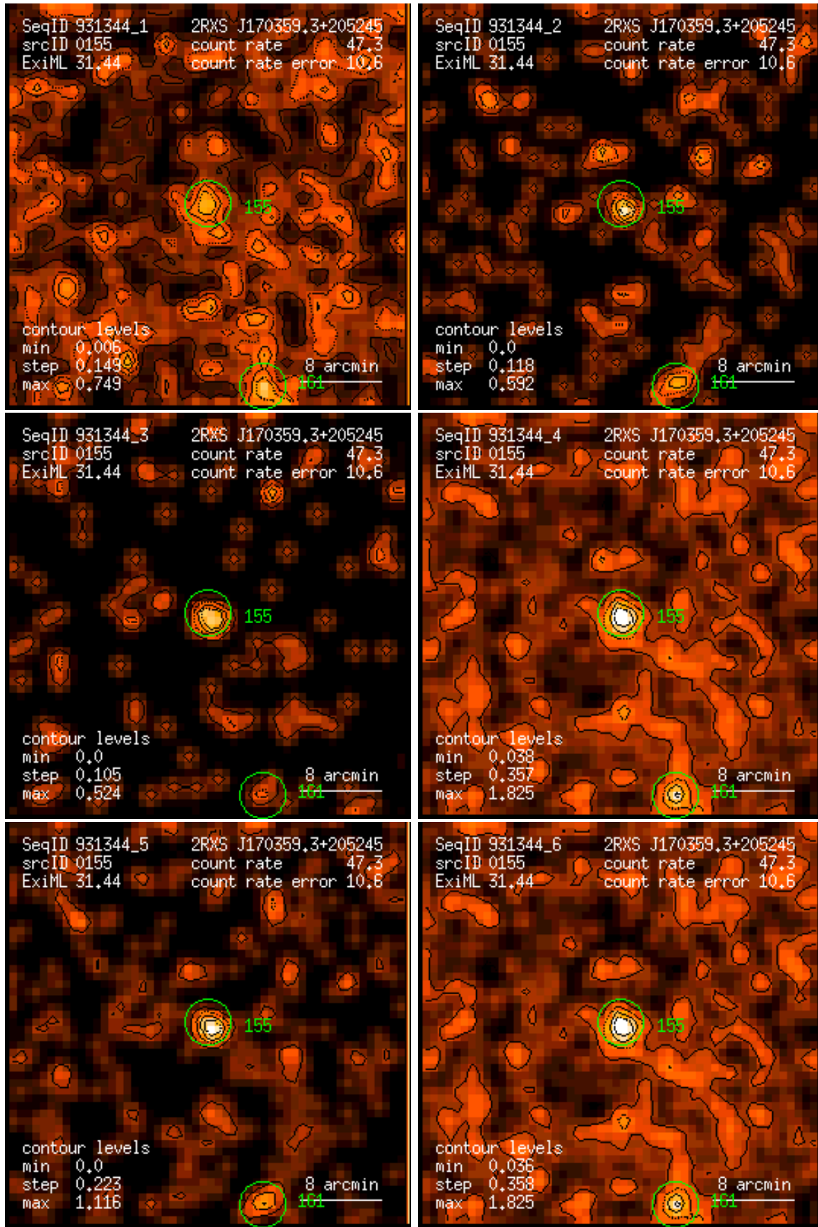
Figure 155: RASS 931344: detection 0155: band rate images, Gaussian filter: (1) PSPC channels 11 – 41, (2) 52 – 90, (3) 91 – 201, (4) 11 – 235, (5) 52 – 201, (6) 11 – 201. Broad band rates in counts/ks. Band rate contour levels in counts/ks/arcmin 2 .
