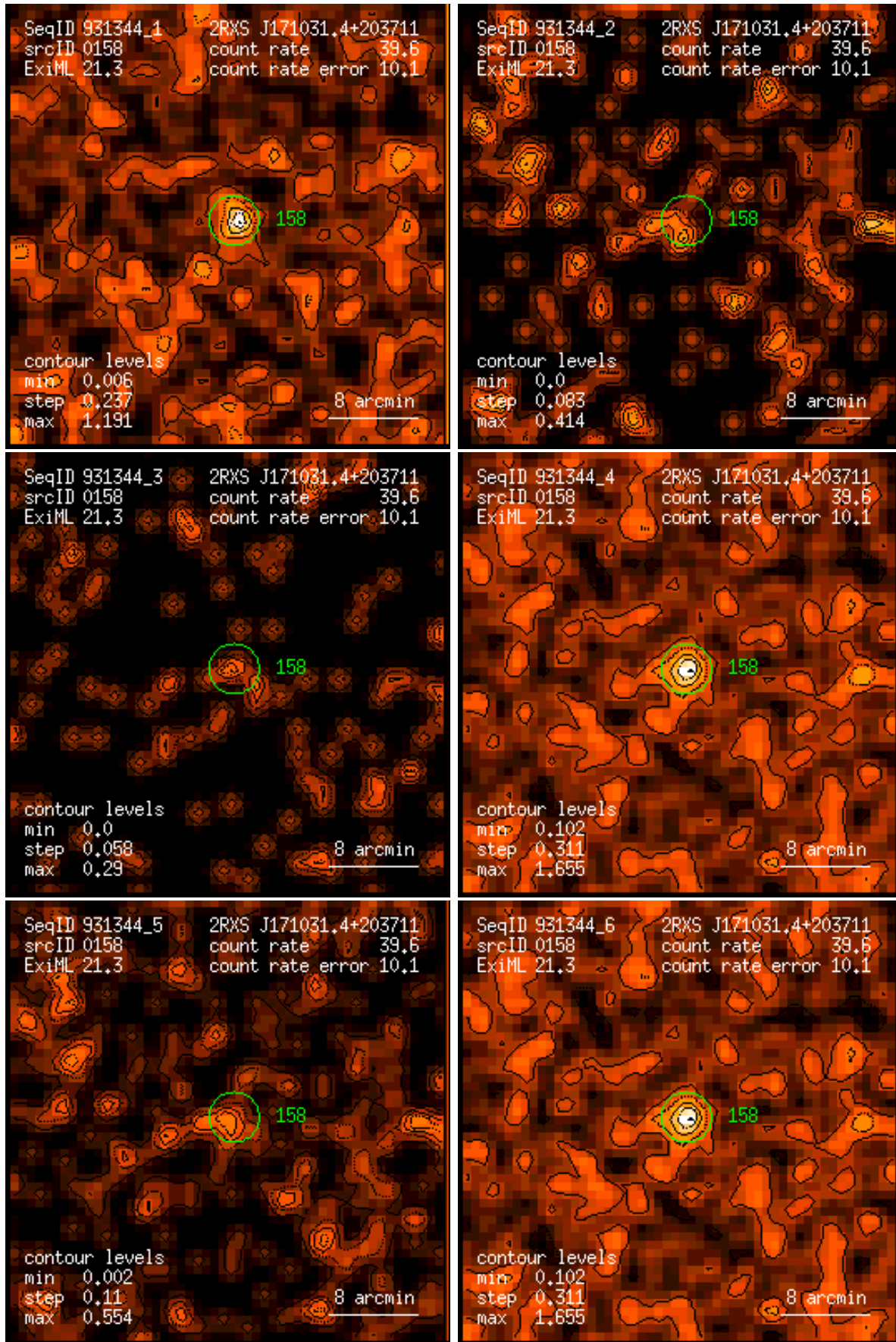
Figure 158: RASS 931344: detection 0158: band rate images, Gaussian filter: (1) PSPC channels 11 – 41, (2) 52 – 90, (3) 91 – 201, (4) 11 – 235, (5) 52 – 201, (6) 11 – 201. Broad band rates in counts/ks. Band rate contour levels in counts/ks/arcmin 2 .
