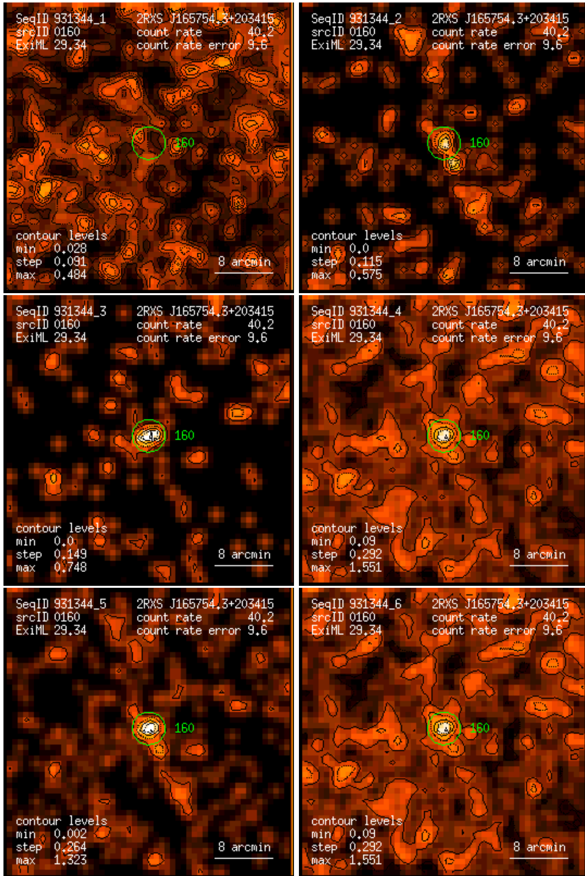
Figure 160: RASS 931344: detection 0160: band rate images, Gaussian filter: (1) PSPC channels 11 – 41, (2) 52 – 90, (3) 91 – 201, (4) 11 – 235, (5) 52 – 201, (6) 11 – 201. Broad band rates in counts/ks. Band rate contour levels in counts/ks/arcmin 2 .
