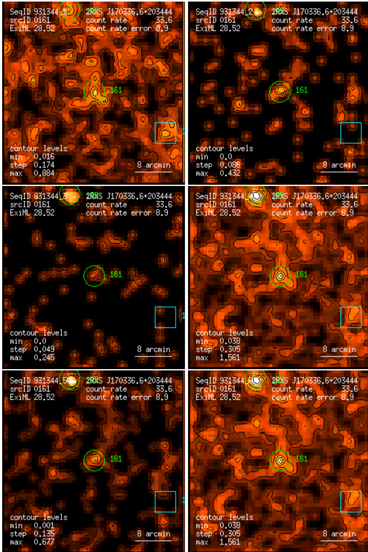
Figure 161: RASS 931344: detection 0161: band rate images, Gaussian filter: (1) PSPC channels 11 – 41, (2) 52 – 90, (3) 91 – 201, (4) 11 – 235, (5) 52 – 201, (6) 11 – 201. Broad band rates in counts/ks. Band rate contour levels in counts/ks/arcmin 2 .
