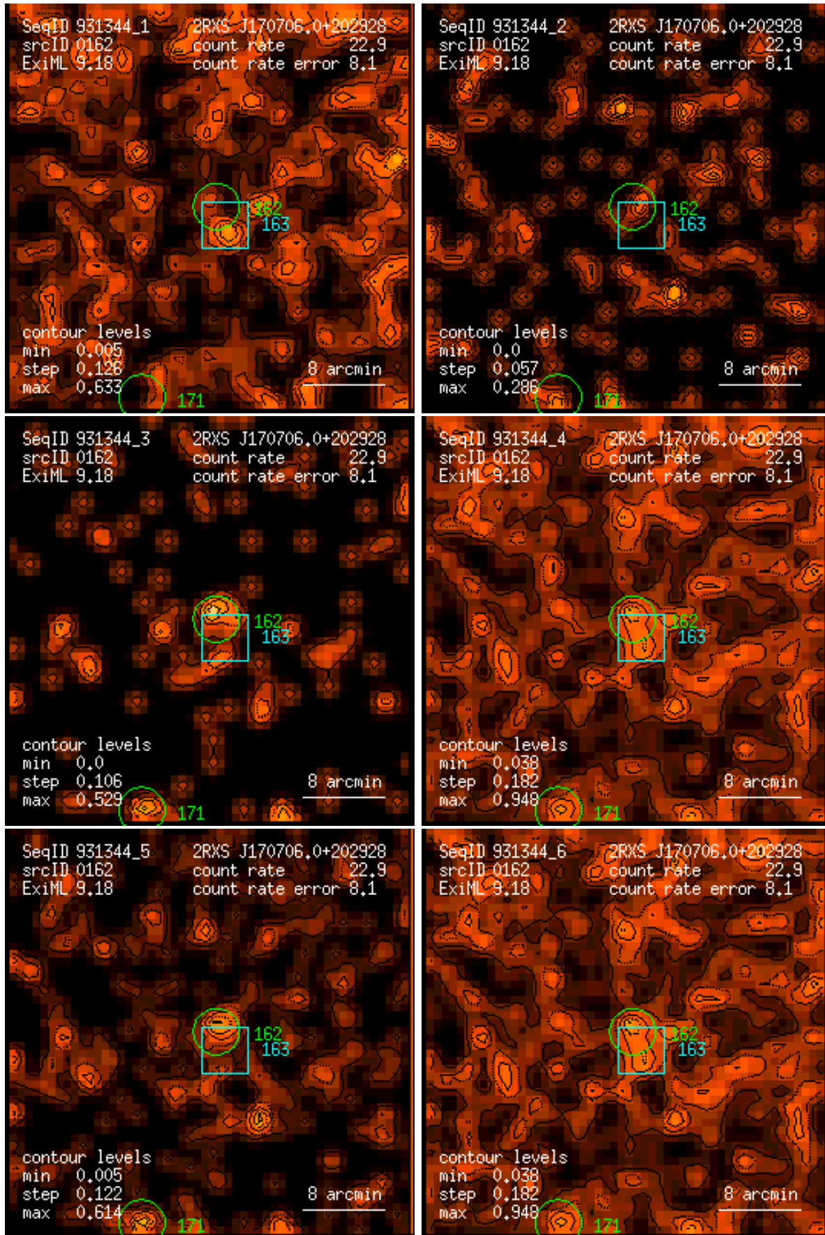
Figure 162: RASS 931344: detection 0162: band rate images, Gaussian filter: (1) PSPC channels 11 – 41, (2) 52 – 90, (3) 91 – 201, (4) 11 – 235, (5) 52 – 201, (6) 11 – 201. Broad band rates in counts/ks. Band rate contour levels in counts/ks/arcmin 2 .
