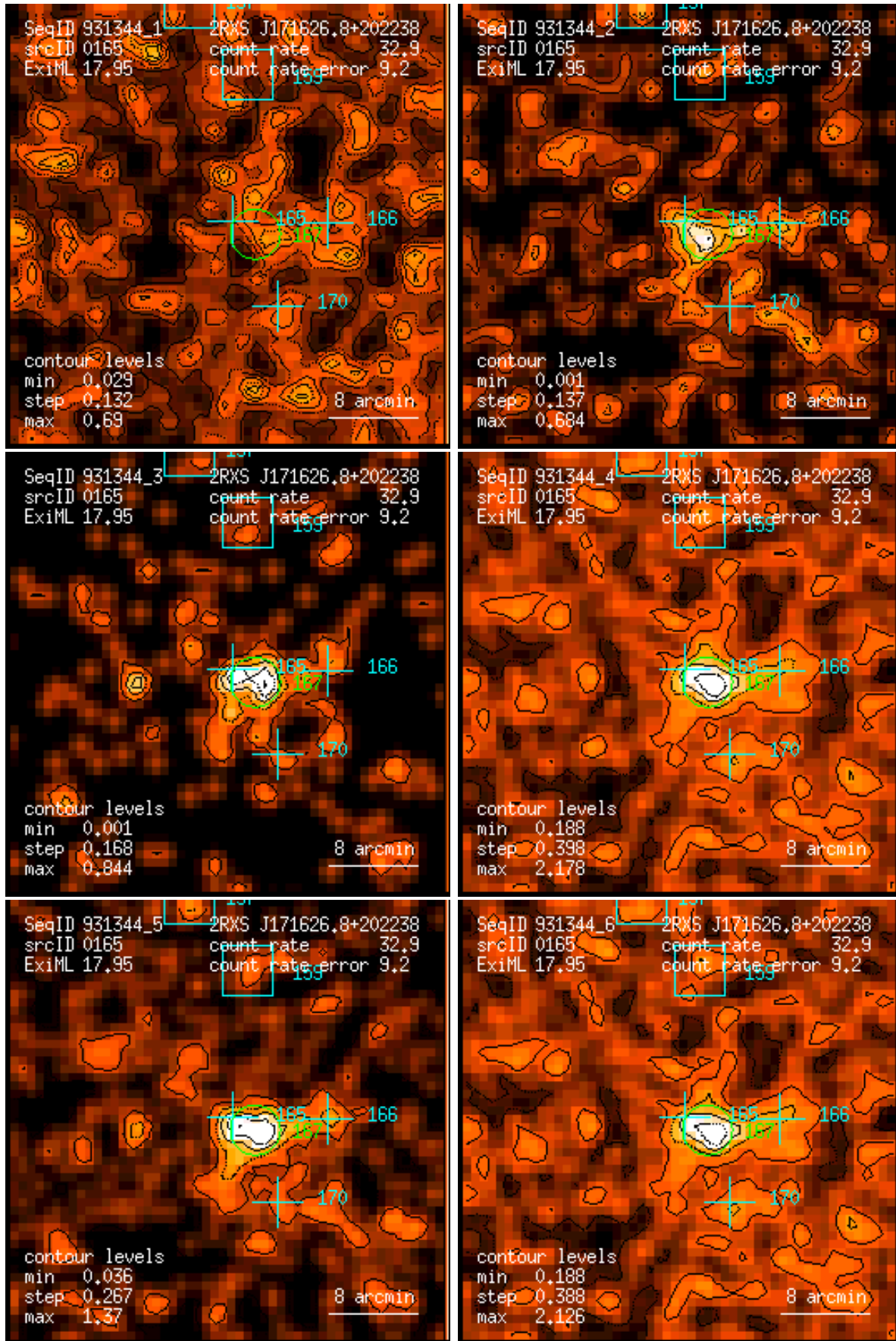
Figure 165: RASS 931344: detection 0165: band rate images, Gaussian filter: (1) PSPC channels 11 – 41, (2) 52 – 90, (3) 91 – 201, (4) 11 – 235, (5) 52 – 201, (6) 11 – 201. Broad band rates in counts/ks. Band rate contour levels in counts/ks/arcmin 2 .
