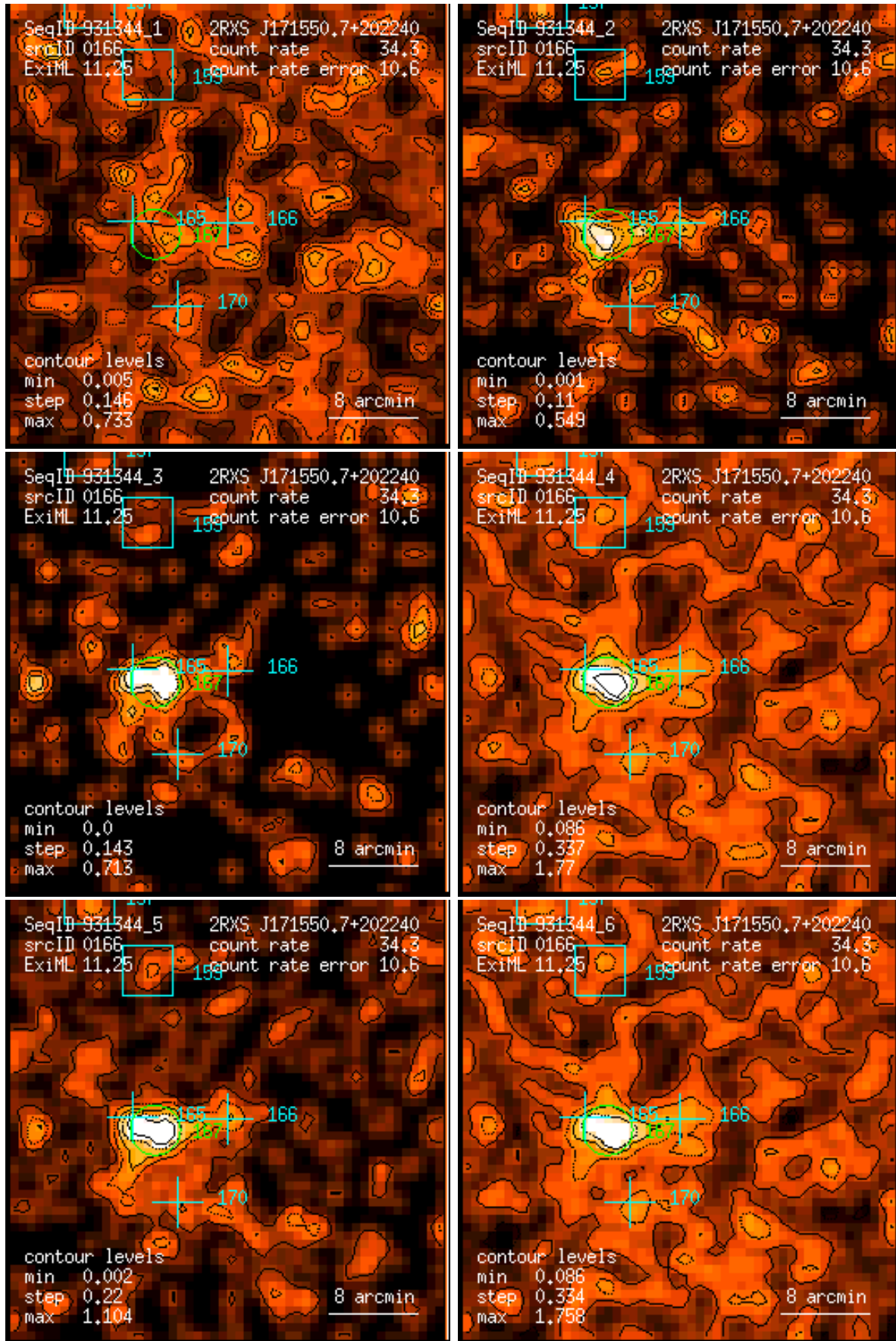
Figure 166: RASS 931344: detection 0166: band rate images, Gaussian filter: (1) PSPC channels 11 – 41, (2) 52 – 90, (3) 91 – 201, (4) 11 – 235, (5) 52 – 201, (6) 11 – 201. Broad band rates in counts/ks. Band rate contour levels in counts/ks/arcmin 2 .
