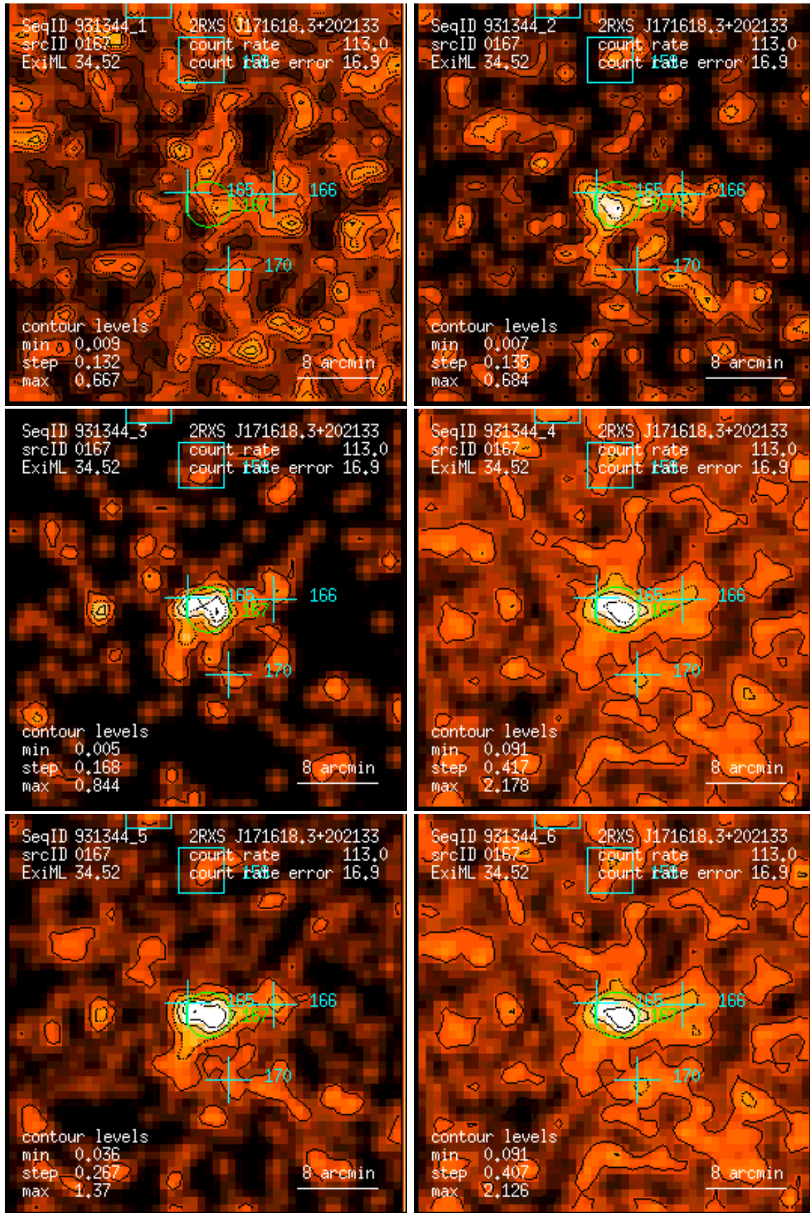
Figure 167: RASS 931344: detection 0167: band rate images, Gaussian filter: (1) PSPC channels 11 – 41, (2) 52 – 90, (3) 91 – 201, (4) 11 – 235, (5) 52 – 201, (6) 11 – 201. Broad band rates in counts/ks. Band rate contour levels in counts/ks/arcmin 2 .
