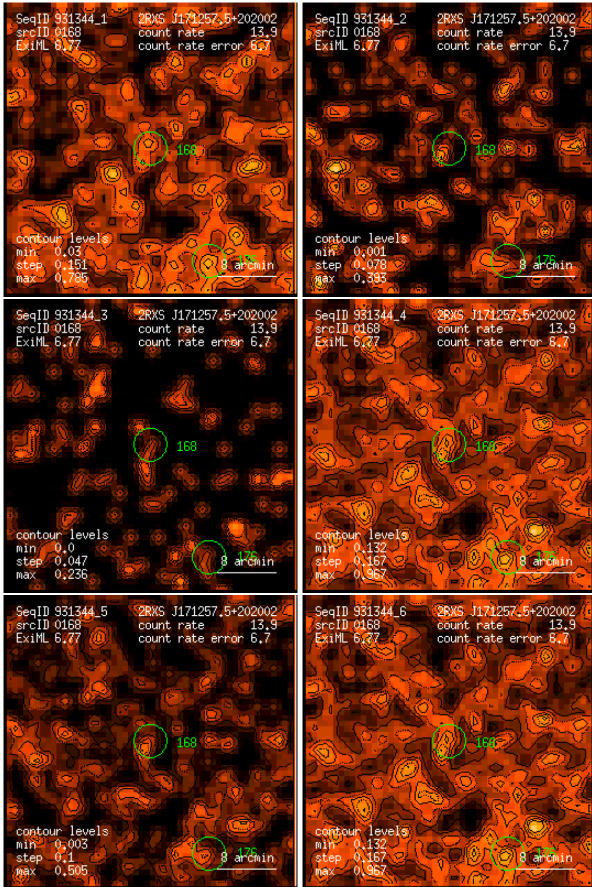
Figure 168: RASS 931344: detection 0168: band rate images, Gaussian filter: (1) PSPC channels 11 – 41, (2) 52 – 90, (3) 91 – 201, (4) 11 – 235, (5) 52 – 201, (6) 11 – 201. Broad band rates in counts/ks. Band rate contour levels in counts/ks/arcmin 2 .
