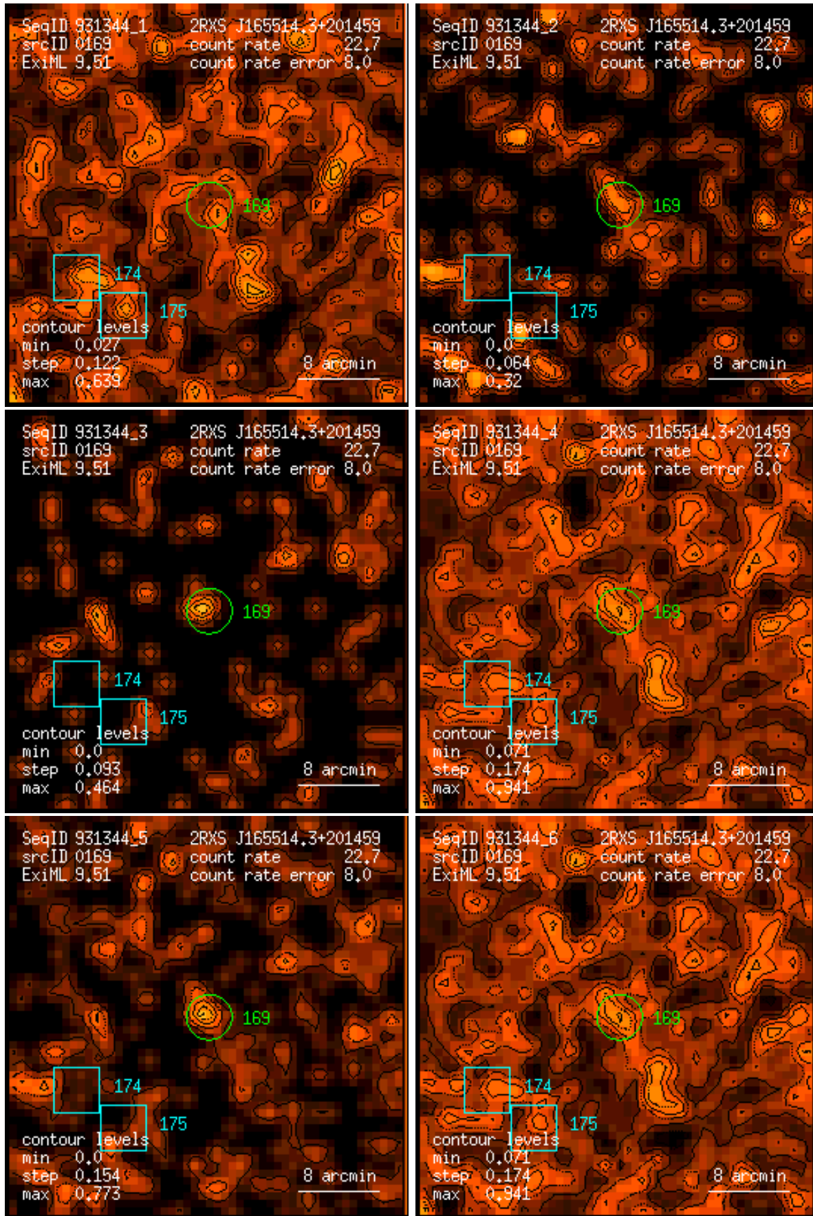
Figure 169: RASS 931344: detection 0169: band rate images, Gaussian filter: (1) PSPC channels 11 – 41, (2) 52 – 90, (3) 91 – 201, (4) 11 – 235, (5) 52 – 201, (6) 11 – 201. Broad band rates in counts/ks. Band rate contour levels in counts/ks/arcmin 2 .
