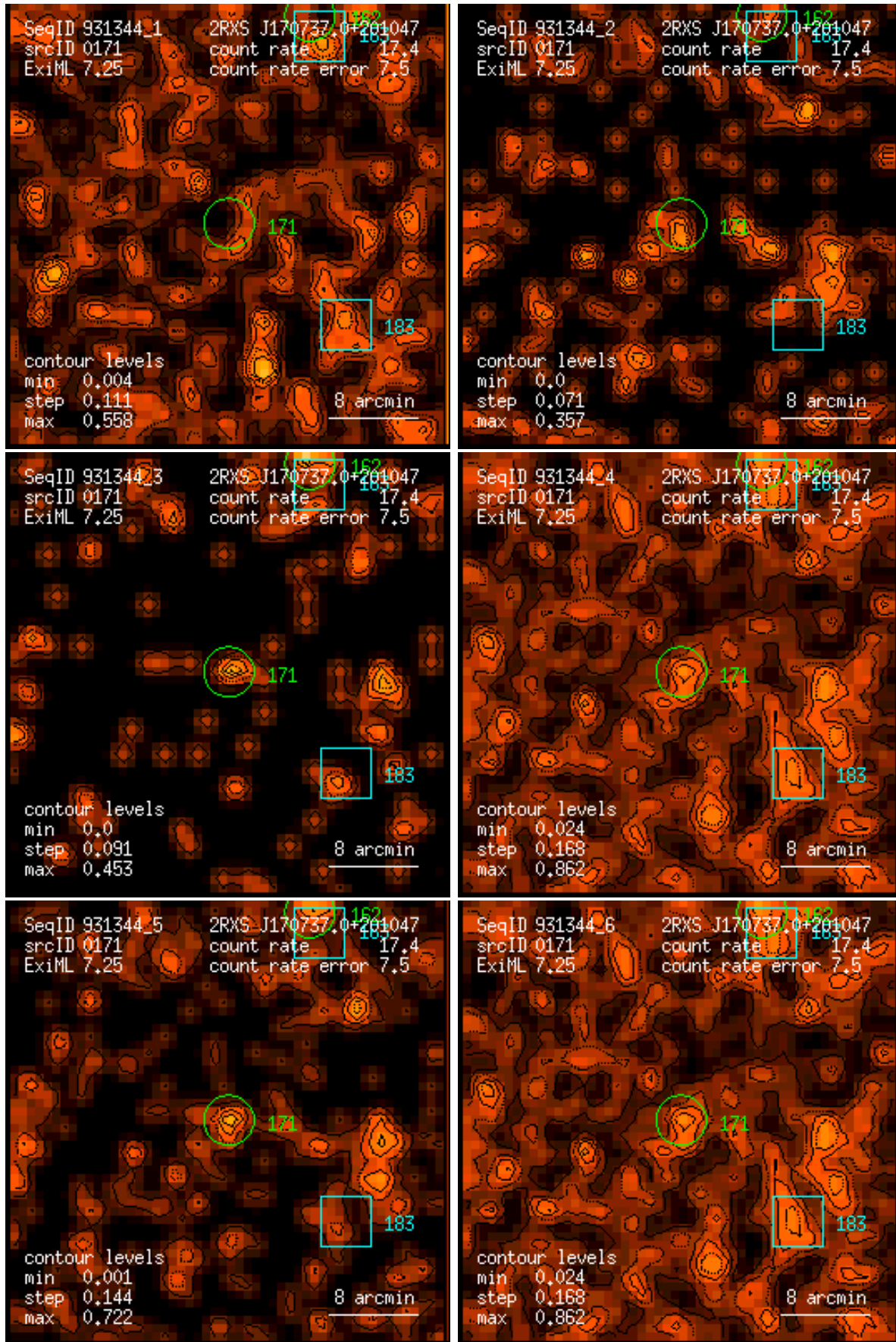
Figure 171: RASS 931344: detection 0171: band rate images, Gaussian filter: (1) PSPC channels 11 – 41, (2) 52 – 90, (3) 91 – 201, (4) 11 – 235, (5) 52 – 201, (6) 11 – 201. Broad band rates in counts/ks. Band rate contour levels in counts/ks/arcmin 2 .
