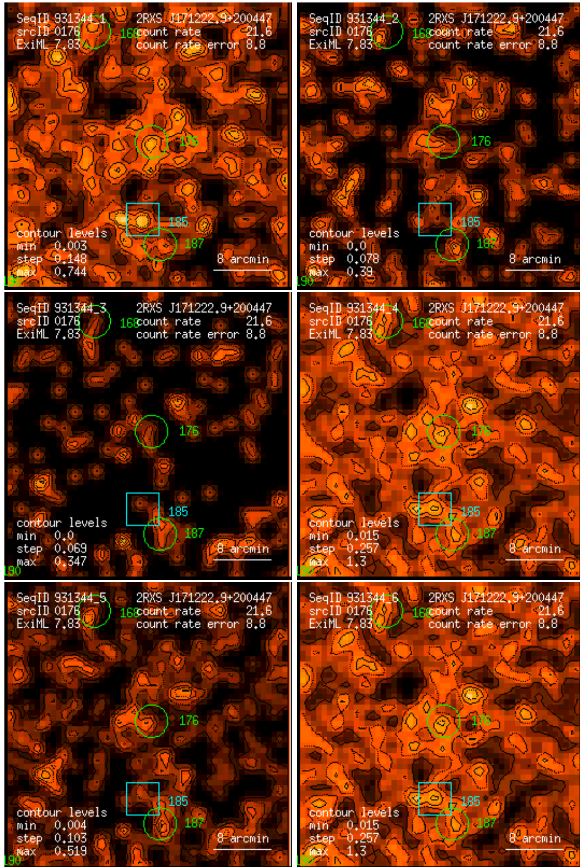
Figure 176: RASS 931344: detection 0176: band rate images, Gaussian filter: (1) PSPC channels 11 – 41, (2) 52 – 90, (3) 91 – 201, (4) 11 – 235, (5) 52 – 201, (6) 11 – 201. Broad band rates in counts/ks. Band rate contour levels in counts/ks/arcmin 2 .
