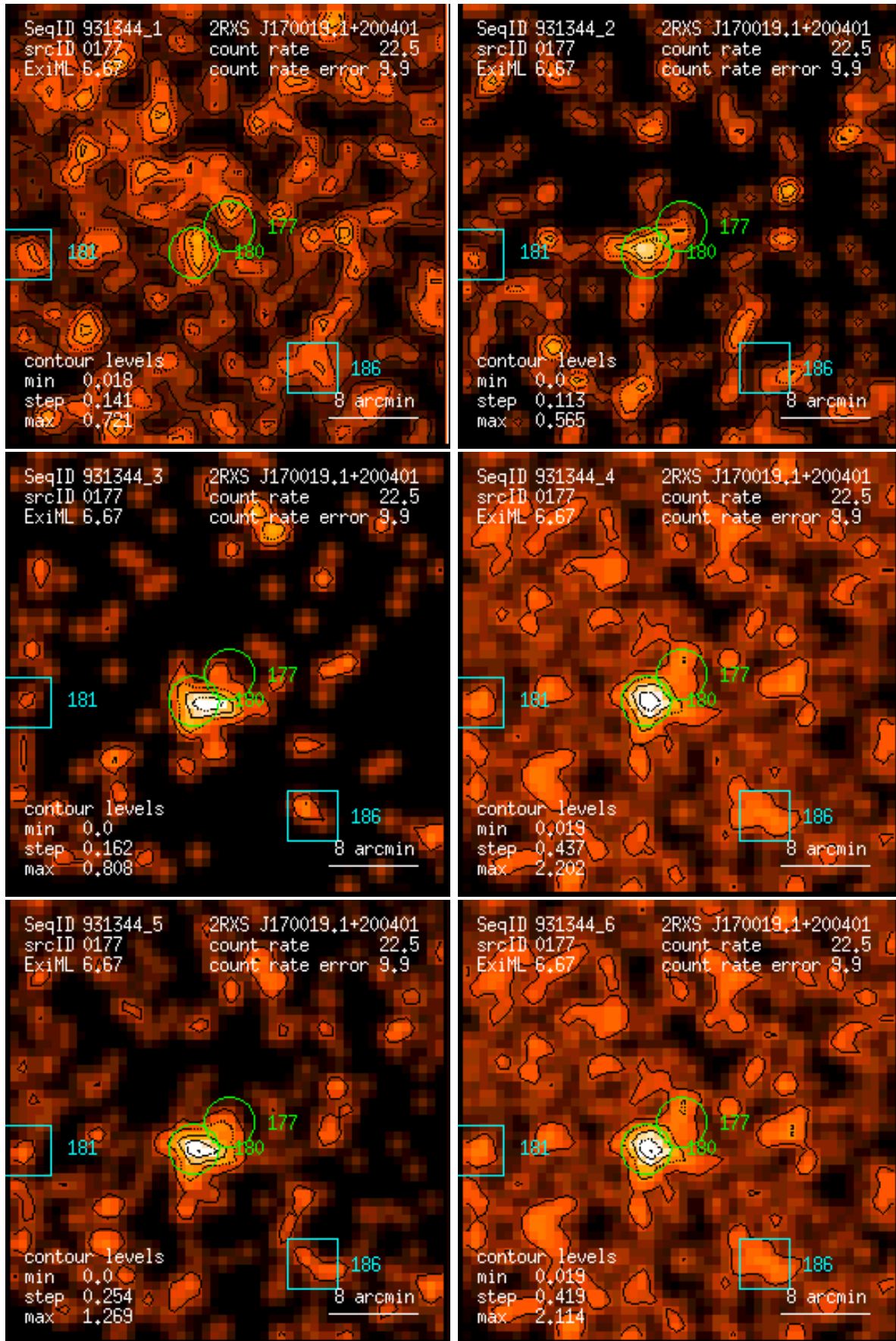
Figure 177: RASS 931344: detection 0177: band rate images, Gaussian filter: (1) PSPC channels 11 – 41, (2) 52 – 90, (3) 91 – 201, (4) 11 – 235, (5) 52 – 201, (6) 11 – 201. Broad band rates in counts/ks. Band rate contour levels in counts/ks/arcmin 2 .
