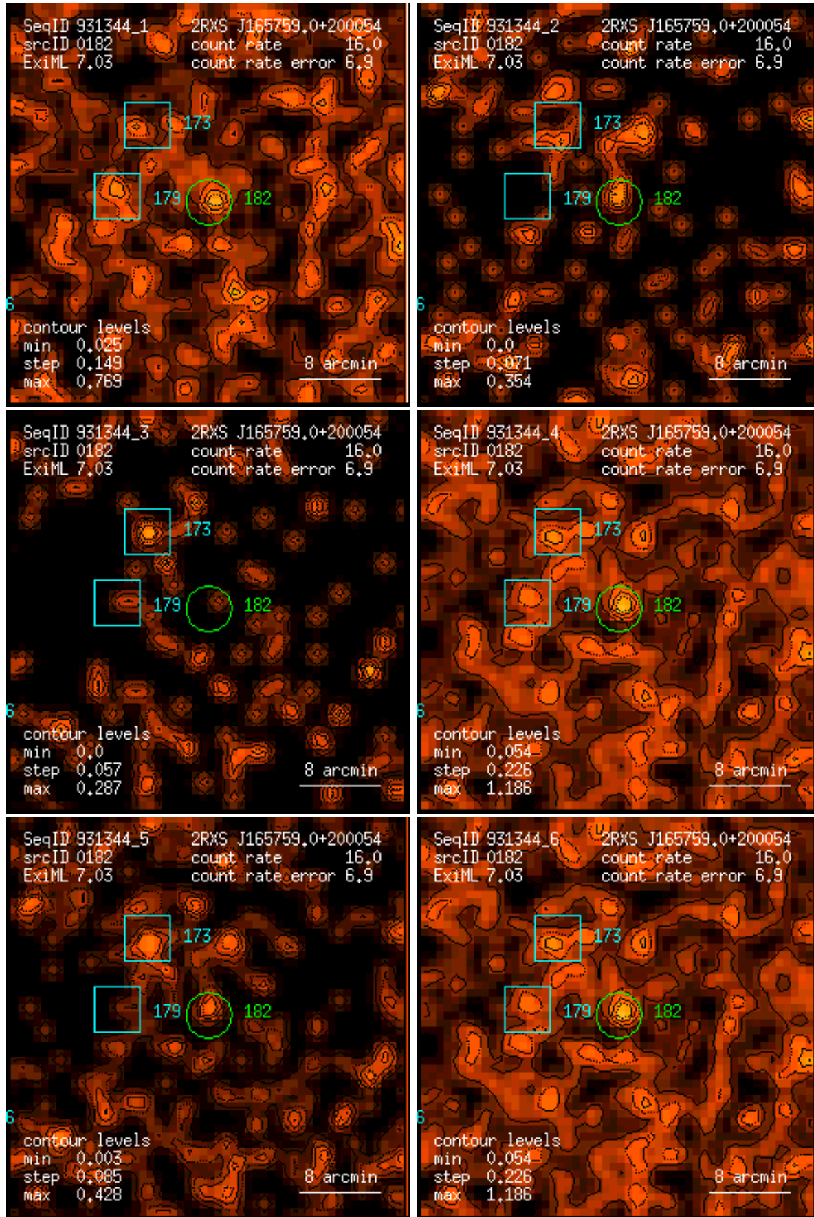
Figure 182: RASS 931344: detection 0182: band rate images, Gaussian filter: (1) PSPC channels 11 – 41, (2) 52 – 90, (3) 91 – 201, (4) 11 – 235, (5) 52 – 201, (6) 11 – 201. Broad band rates in counts/ks. Band rate contour levels in counts/ks/arcmin 2 .
