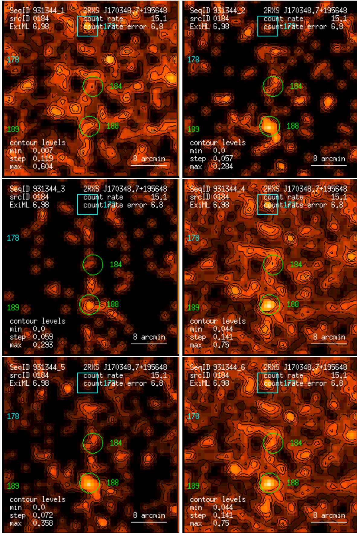
Figure 184: RASS 931344: detection 0184: band rate images, Gaussian filter: (1) PSPC channels 11 – 41, (2) 52 – 90, (3) 91 – 201, (4) 11 – 235, (5) 52 – 201, (6) 11 – 201. Broad band rates in counts/ks. Band rate contour levels in counts/ks/arcmin 2 .
