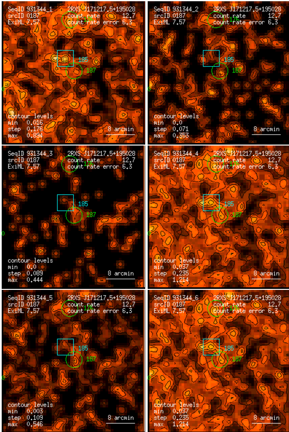
Figure 187: RASS 931344: detection 0187: band rate images, Gaussian filter: (1) PSPC channels 11 – 41, (2) 52 – 90, (3) 91 – 201, (4) 11 – 235, (5) 52 – 201, (6) 11 – 201. Broad band rates in counts/ks. Band rate contour levels in counts/ks/arcmin 2 .
