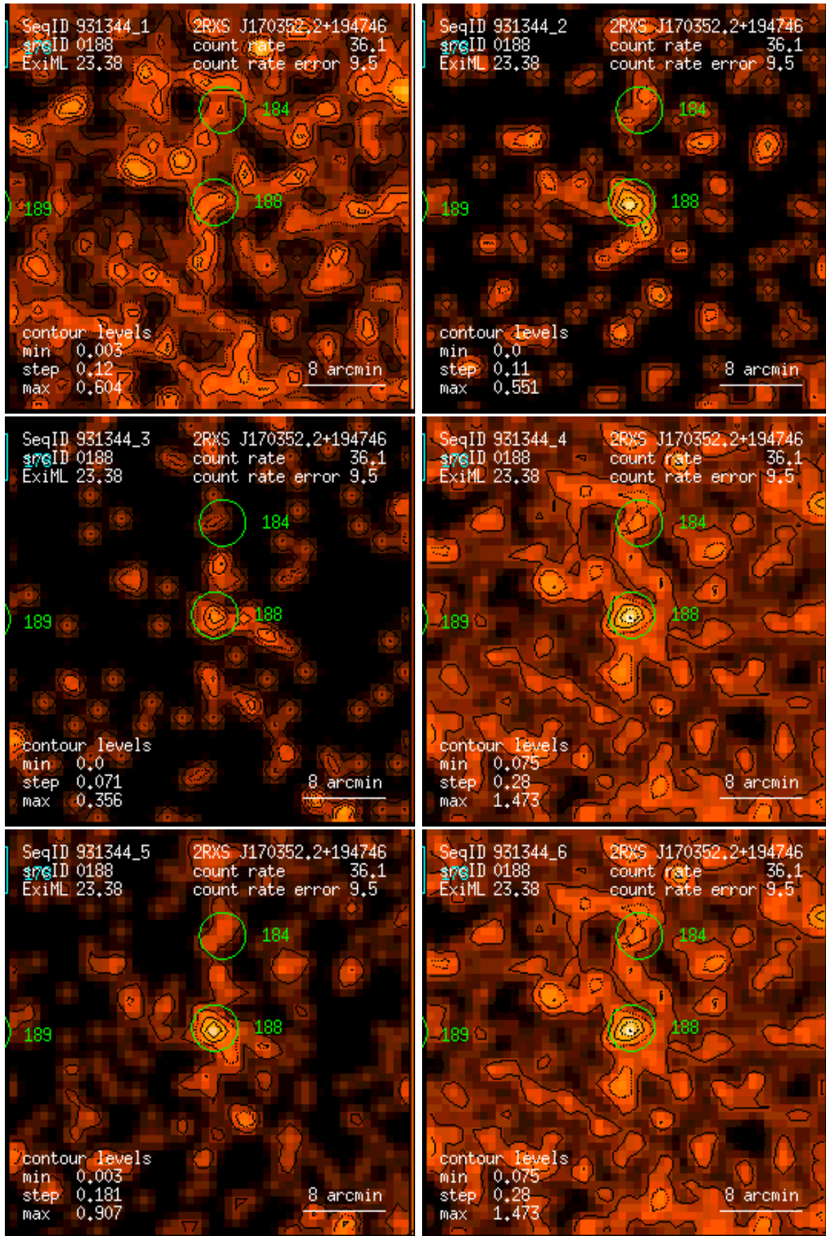
Figure 188: RASS 931344: detection 0188: band rate images, Gaussian filter: (1) PSPC channels 11 – 41, (2) 52 – 90, (3) 91 – 201, (4) 11 – 235, (5) 52 – 201, (6) 11 – 201. Broad band rates in counts/ks. Band rate contour levels in counts/ks/arcmin 2 .
