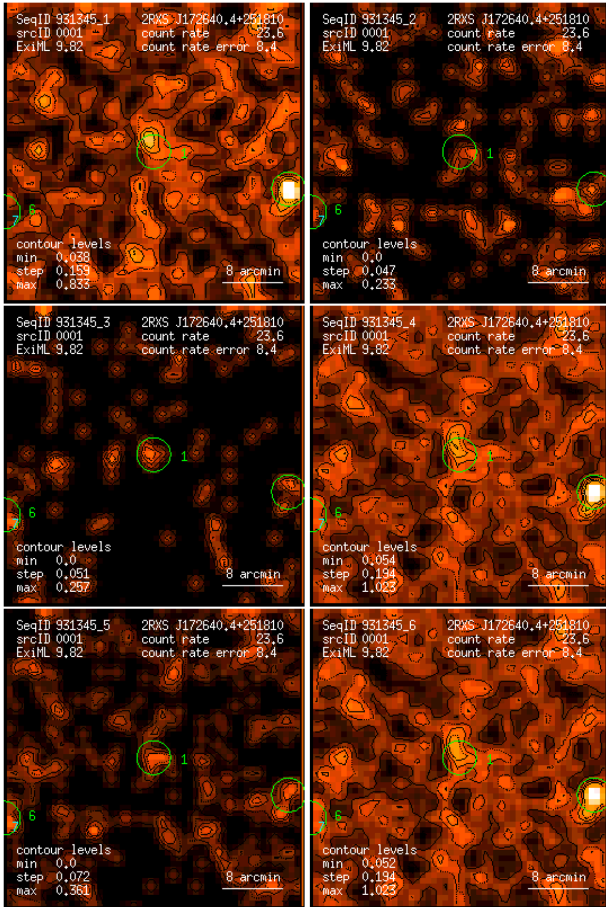
Figure 1: RASS 931345: detection 0001: band rate images, Gaussian filter: (1) PSPC channels 11 – 41, (2) 52 – 90, (3) 91 – 201, (4) 11 – 235, (5) 52 – 201, (6) 11 – 201. Broad band rates in counts/ks. Band rate contour levels in counts/ks/arcmin 2 .
