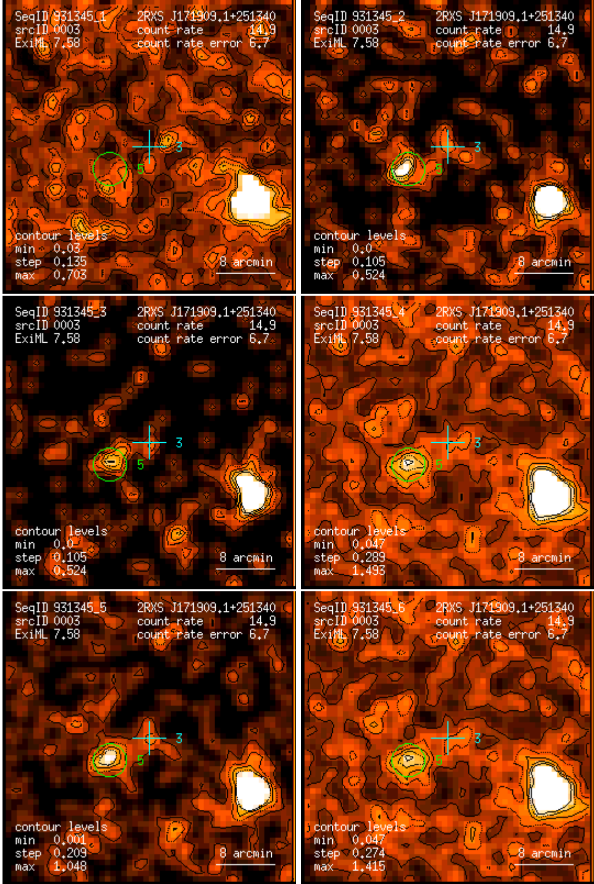
Figure 3: RASS 931345: detection 0003: band rate images, Gaussian filter: (1) PSPC channels 11 – 41, (2) 52 – 90, (3) 91 – 201, (4) 11 – 235, (5) 52 – 201, (6) 11 – 201. Broad band rates in counts/ks. Band rate contour levels in counts/ks/arcmin 2 .
