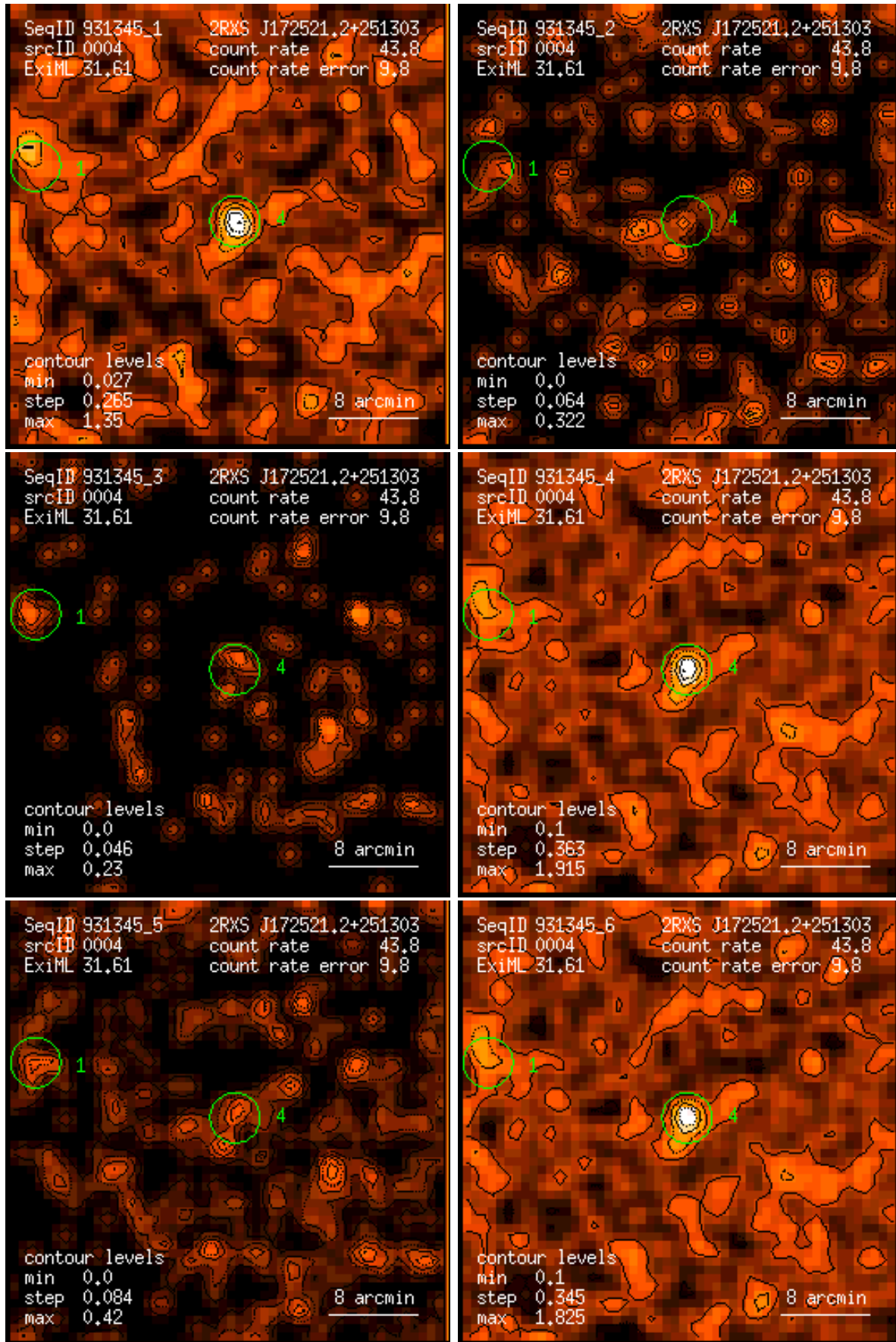
Figure 4: RASS 931345: detection 0004: band rate images, Gaussian filter: (1) PSPC channels 11 – 41, (2) 52 – 90, (3) 91 – 201, (4) 11 – 235, (5) 52 – 201, (6) 11 – 201. Broad band rates in counts/ks. Band rate contour levels in counts/ks/arcmin 2 .
