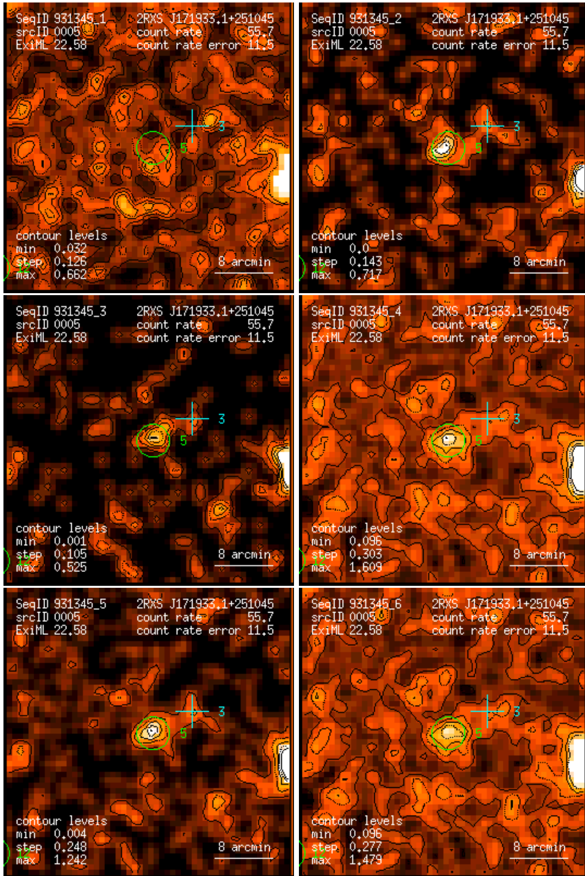
Figure 5: RASS 931345: detection 0005: band rate images, Gaussian filter: (1) PSPC channels 11 – 41, (2) 52 – 90, (3) 91 – 201, (4) 11 – 235, (5) 52 – 201, (6) 11 – 201. Broad band rates in counts/ks. Band rate contour levels in counts/ks/arcmin 2 .
