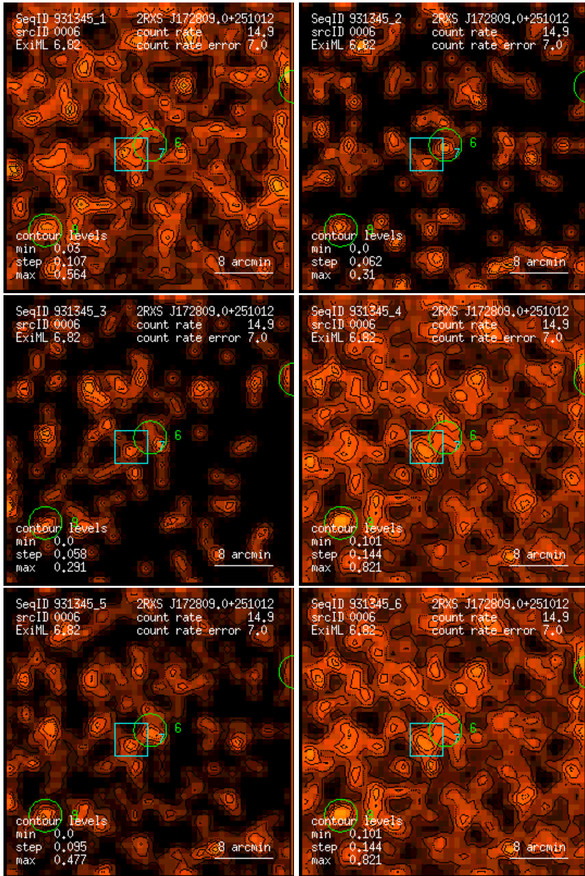
Figure 6: RASS 931345: detection 0006: band rate images, Gaussian filter: (1) PSPC channels 11 – 41, (2) 52 – 90, (3) 91 – 201, (4) 11 – 235, (5) 52 – 201, (6) 11 – 201. Broad band rates in counts/ks. Band rate contour levels in counts/ks/arcmin 2 .
