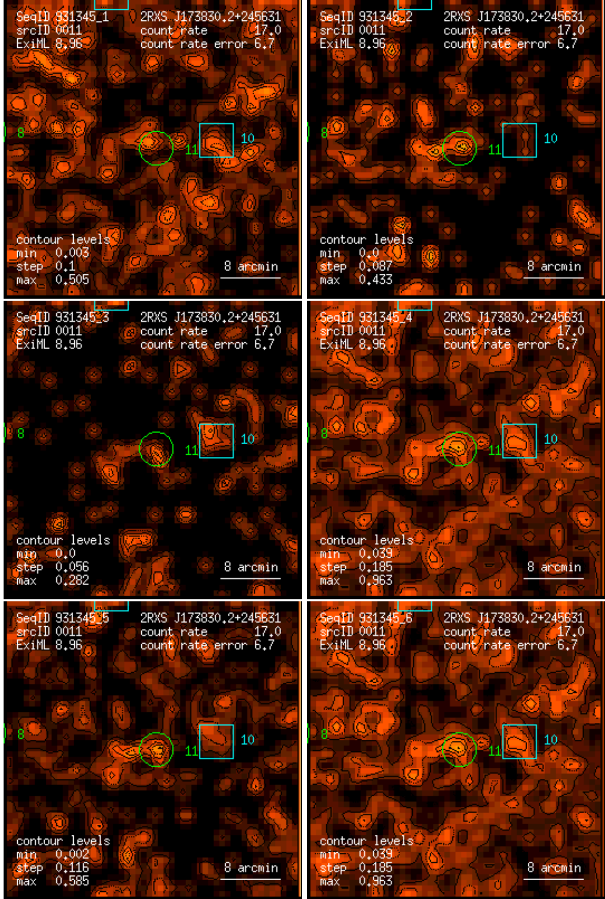
Figure 11: RASS 931345: detection 0011: band rate images, Gaussian filter: (1) PSPC channels 11 – 41, (2) 52 – 90, (3) 91 – 201, (4) 11 – 235, (5) 52 – 201, (6) 11 – 201. Broad band rates in counts/ks. Band rate contour levels in counts/ks/arcmin 2 .
