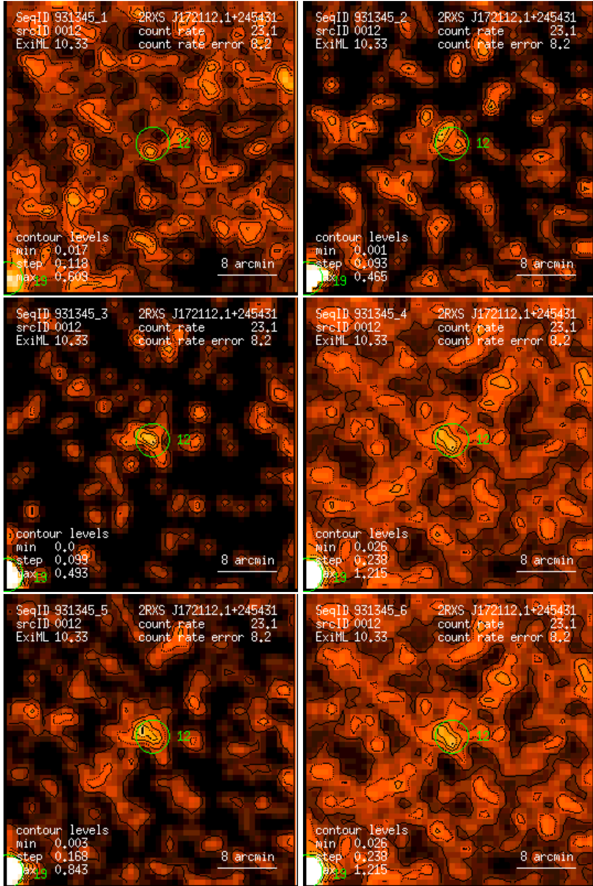
Figure 12: RASS 931345: detection 0012: band rate images, Gaussian filter: (1) PSPC channels 11 – 41, (2) 52 – 90, (3) 91 – 201, (4) 11 – 235, (5) 52 – 201, (6) 11 – 201. Broad band rates in counts/ks. Band rate contour levels in counts/ks/arcmin 2 .
