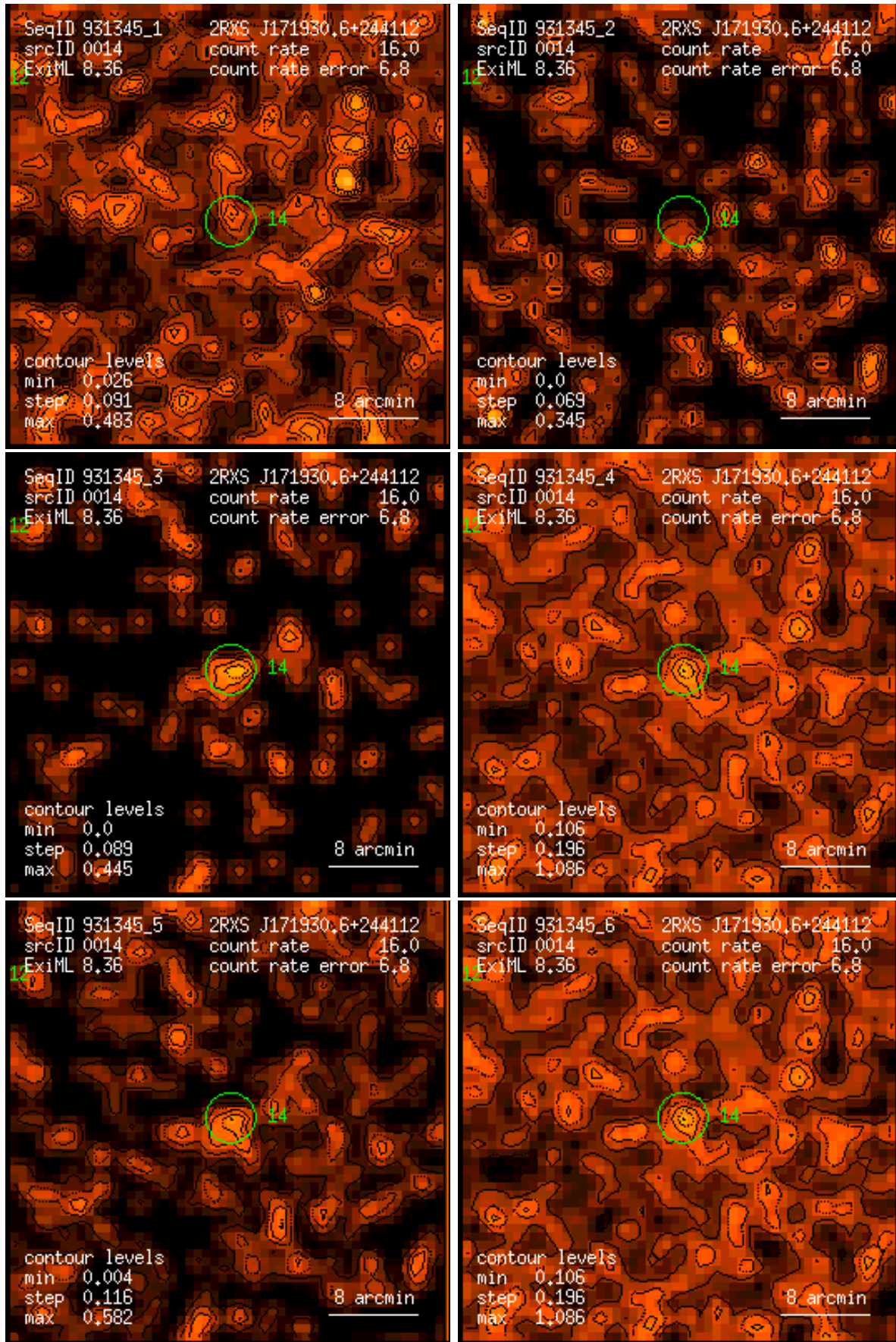
Figure 14: RASS 931345: detection 0014: band rate images, Gaussian filter: (1) PSPC channels 11 – 41, (2) 52 – 90, (3) 91 – 201, (4) 11 – 235, (5) 52 – 201, (6) 11 – 201. Broad band rates in counts/ks. Band rate contour levels in counts/ks/arcmin 2 .
