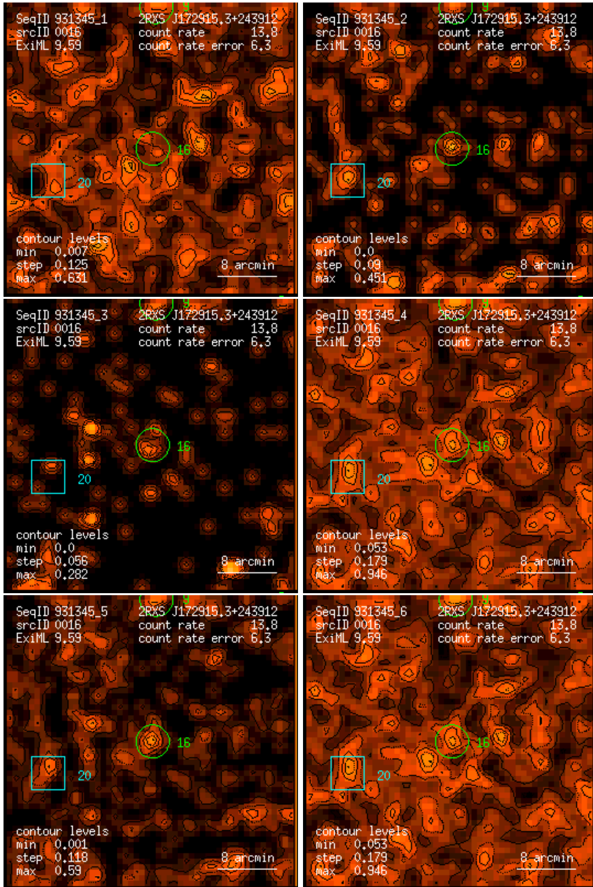
Figure 16: RASS 931345: detection 0016: band rate images, Gaussian filter: (1) PSPC channels 11 – 41, (2) 52 – 90, (3) 91 – 201, (4) 11 – 235, (5) 52 – 201, (6) 11 – 201. Broad band rates in counts/ks. Band rate contour levels in counts/ks/arcmin 2 .
