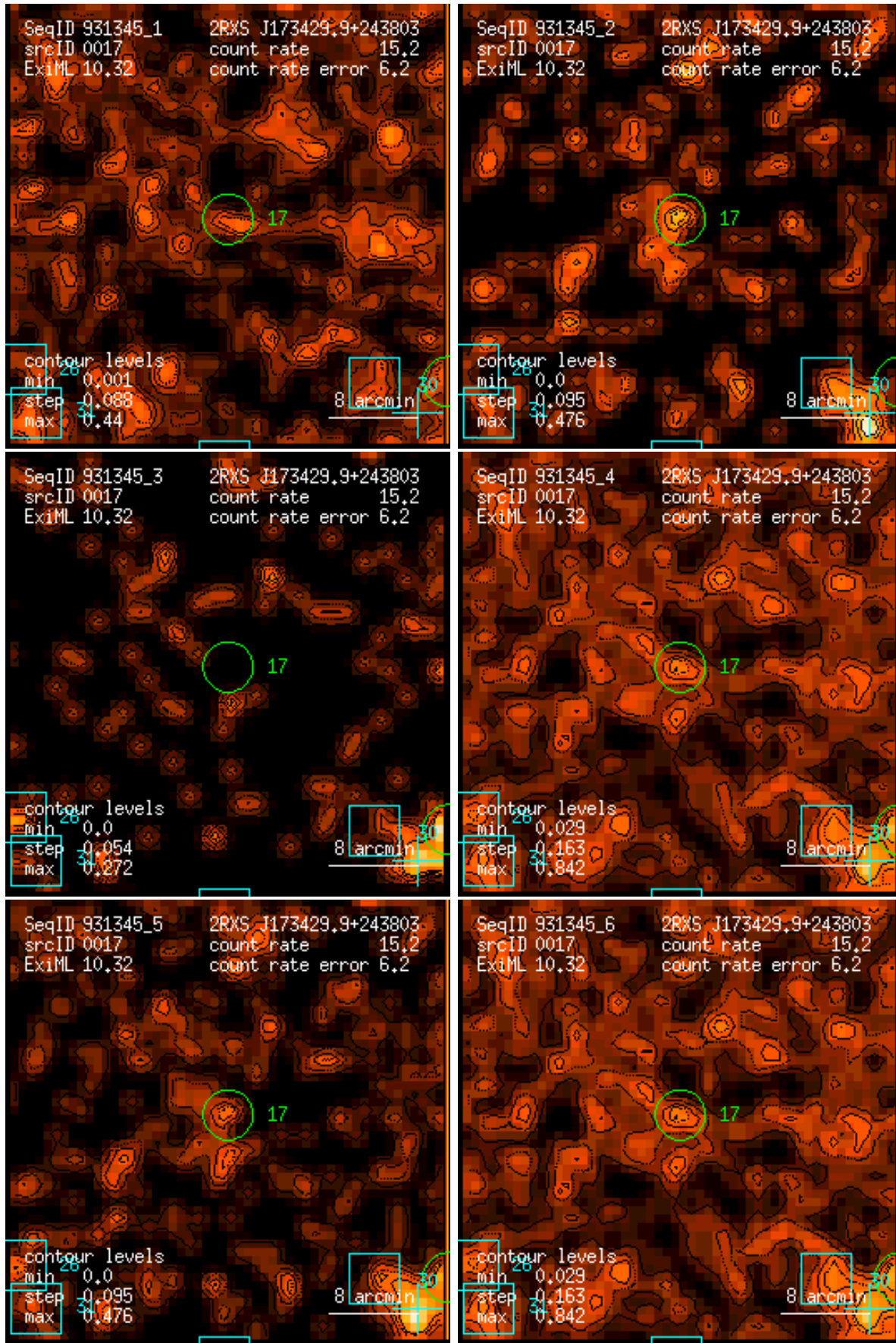
Figure 17: RASS 931345: detection 0017: band rate images, Gaussian filter: (1) PSPC channels 11 – 41, (2) 52 – 90, (3) 91 – 201, (4) 11 – 235, (5) 52 – 201, (6) 11 – 201. Broad band rates in counts/ks. Band rate contour levels in counts/ks/arcmin 2 .
