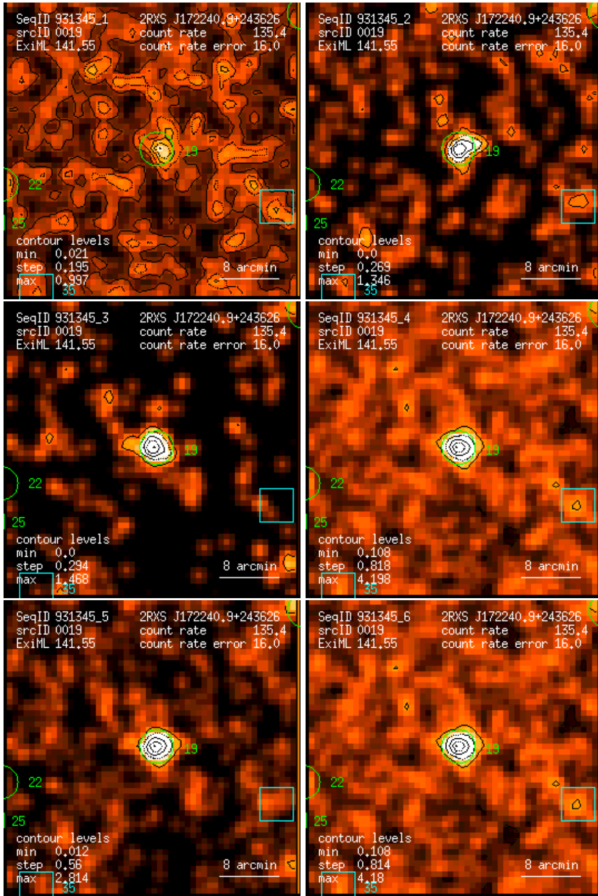
Figure 19: RASS 931345: detection 0019: band rate images, Gaussian filter: (1) PSPC channels 11 – 41, (2) 52 – 90, (3) 91 – 201, (4) 11 – 235, (5) 52 – 201, (6) 11 – 201. Broad band rates in counts/ks. Band rate contour levels in counts/ks/arcmin 2 .
