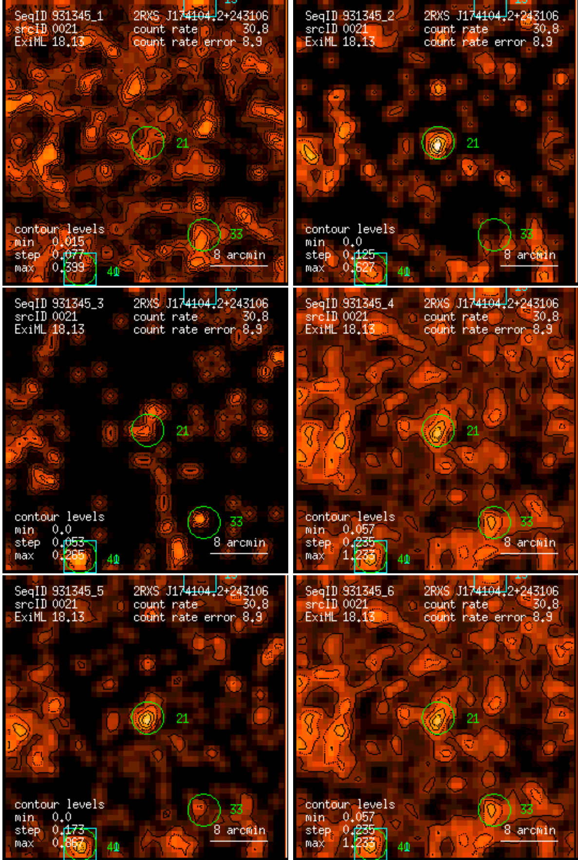
Figure 21: RASS 931345: detection 0021: band rate images, Gaussian filter: (1) PSPC channels 11 – 41, (2) 52 – 90, (3) 91 – 201, (4) 11 – 235, (5) 52 – 201, (6) 11 – 201. Broad band rates in counts/ks. Band rate contour levels in counts/ks/arcmin 2 .
