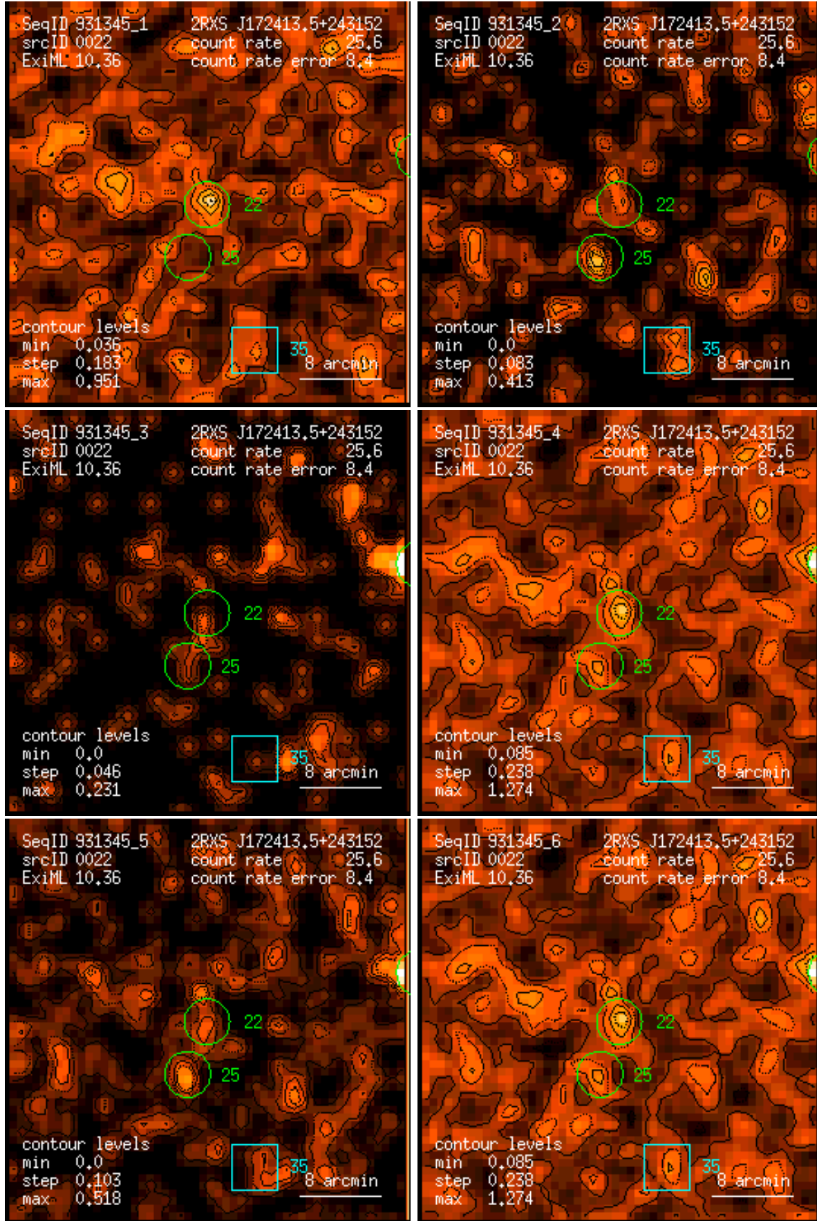
Figure 22: RASS 931345: detection 0022: band rate images, Gaussian filter: (1) PSPC channels 11 – 41, (2) 52 – 90, (3) 91 – 201, (4) 11 – 235, (5) 52 – 201, (6) 11 – 201. Broad band rates in counts/ks. Band rate contour levels in counts/ks/arcmin 2 .
