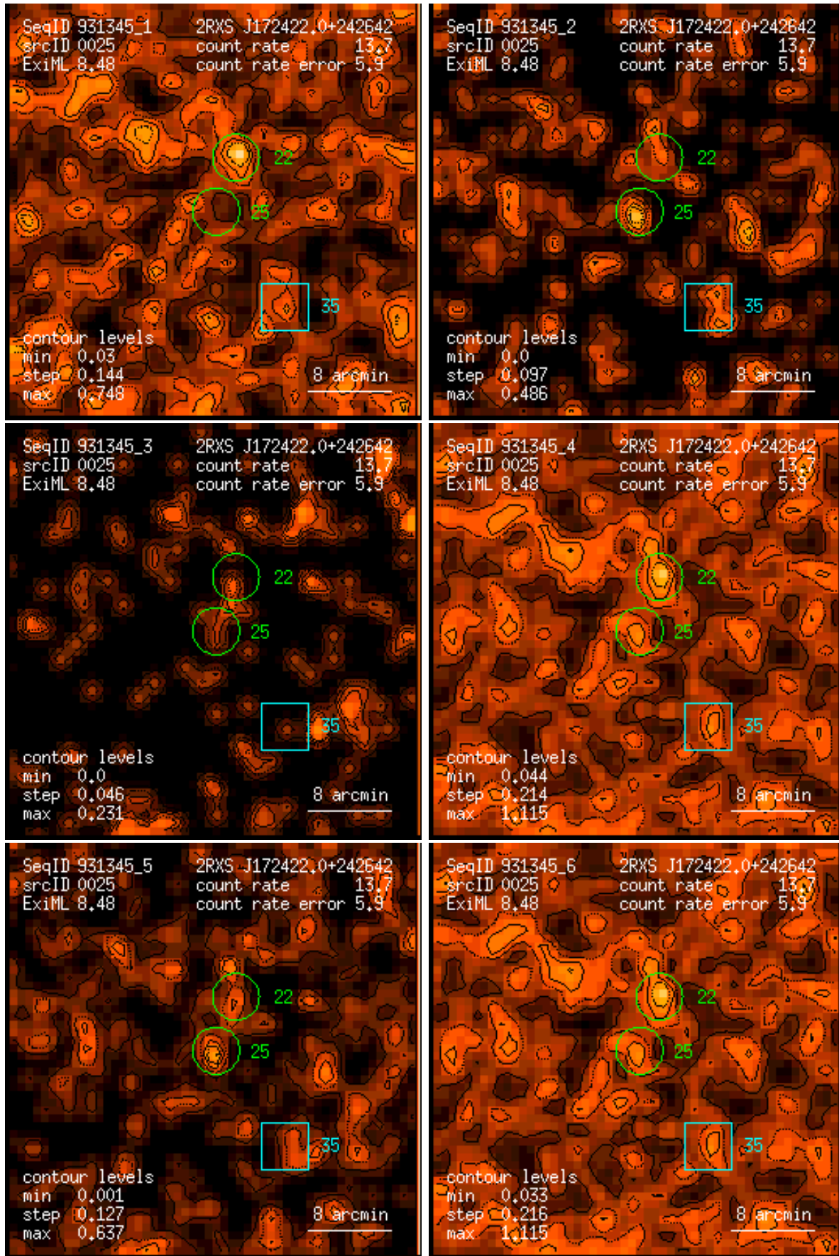
Figure 25: RASS 931345: detection 0025: band rate images, Gaussian filter: (1) PSPC channels 11 – 41, (2) 52 – 90, (3) 91 – 201, (4) 11 – 235, (5) 52 – 201, (6) 11 – 201. Broad band rates in counts/ks. Band rate contour levels in counts/ks/arcmin 2 .
