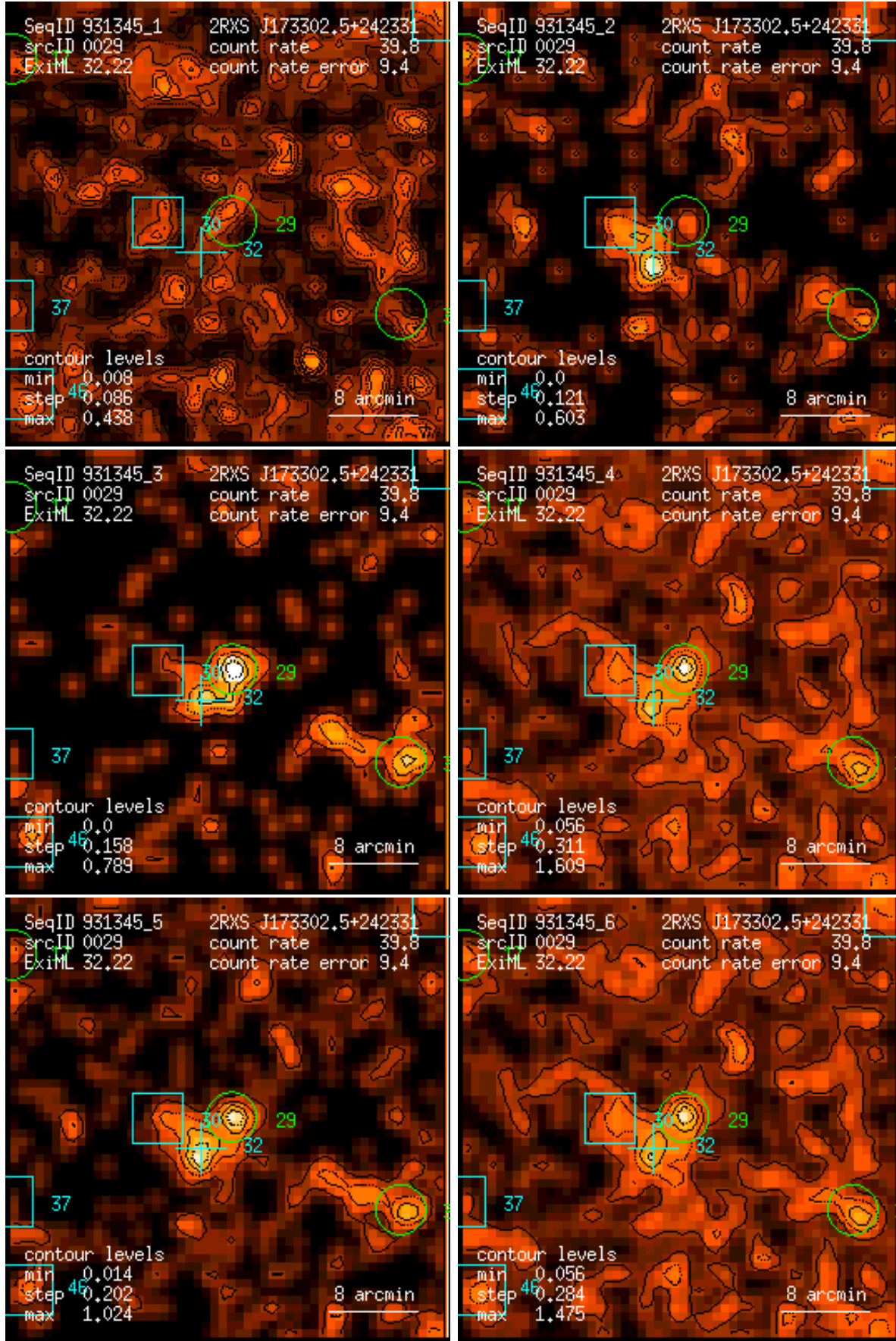
Figure 29: RASS 931345: detection 0029: band rate images, Gaussian filter: (1) PSPC channels 11 – 41, (2) 52 – 90, (3) 91 – 201, (4) 11 – 235, (5) 52 – 201, (6) 11 – 201. Broad band rates in counts/ks. Band rate contour levels in counts/ks/arcmin 2 .
