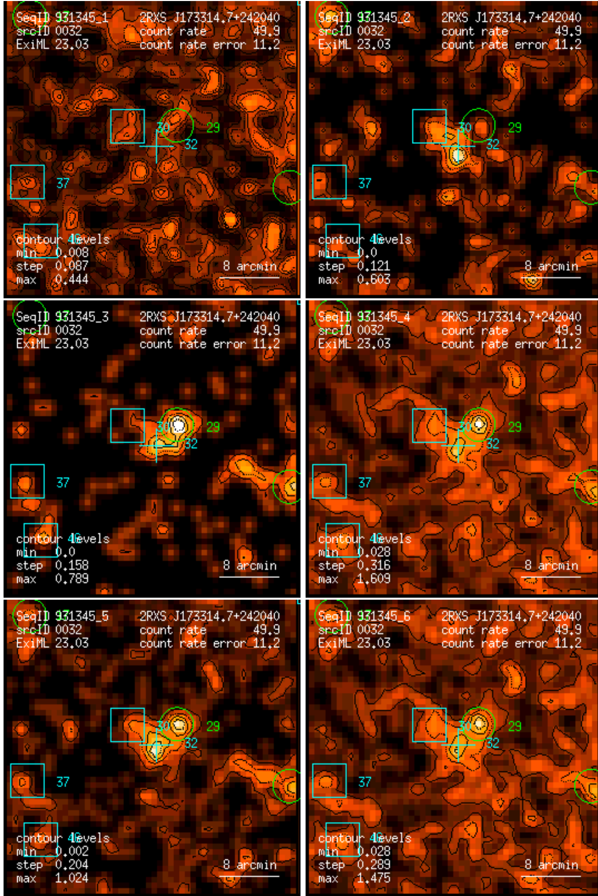
Figure 32: RASS 931345: detection 0032: band rate images, Gaussian filter: (1) PSPC channels 11 – 41, (2) 52 – 90, (3) 91 – 201, (4) 11 – 235, (5) 52 – 201, (6) 11 – 201. Broad band rates in counts/ks. Band rate contour levels in counts/ks/arcmin 2 .
