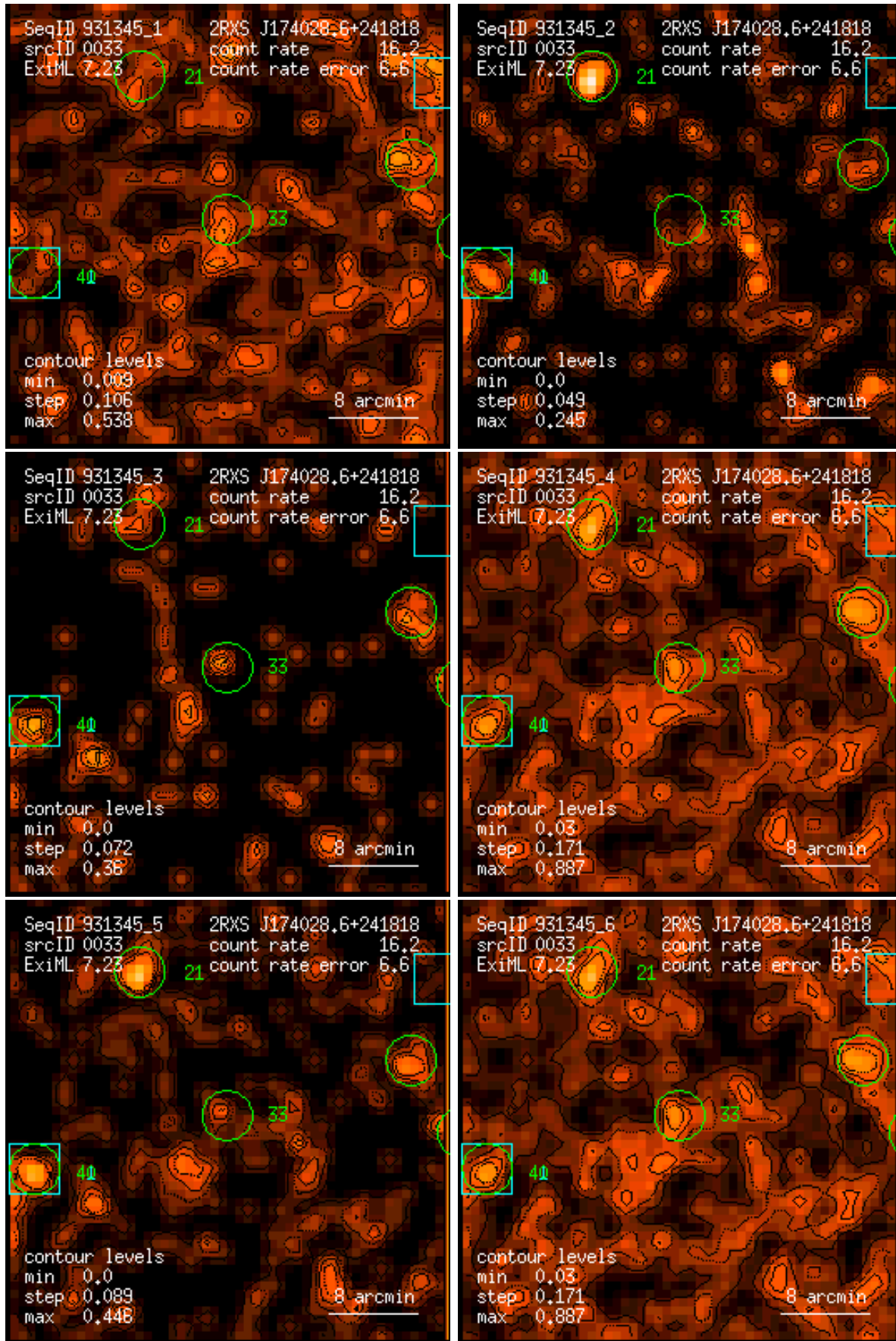
Figure 33: RASS 931345: detection 0033: band rate images, Gaussian filter: (1) PSPC channels 11 – 41, (2) 52 – 90, (3) 91 – 201, (4) 11 – 235, (5) 52 – 201, (6) 11 – 201. Broad band rates in counts/ks. Band rate contour levels in counts/ks/arcmin 2 .
