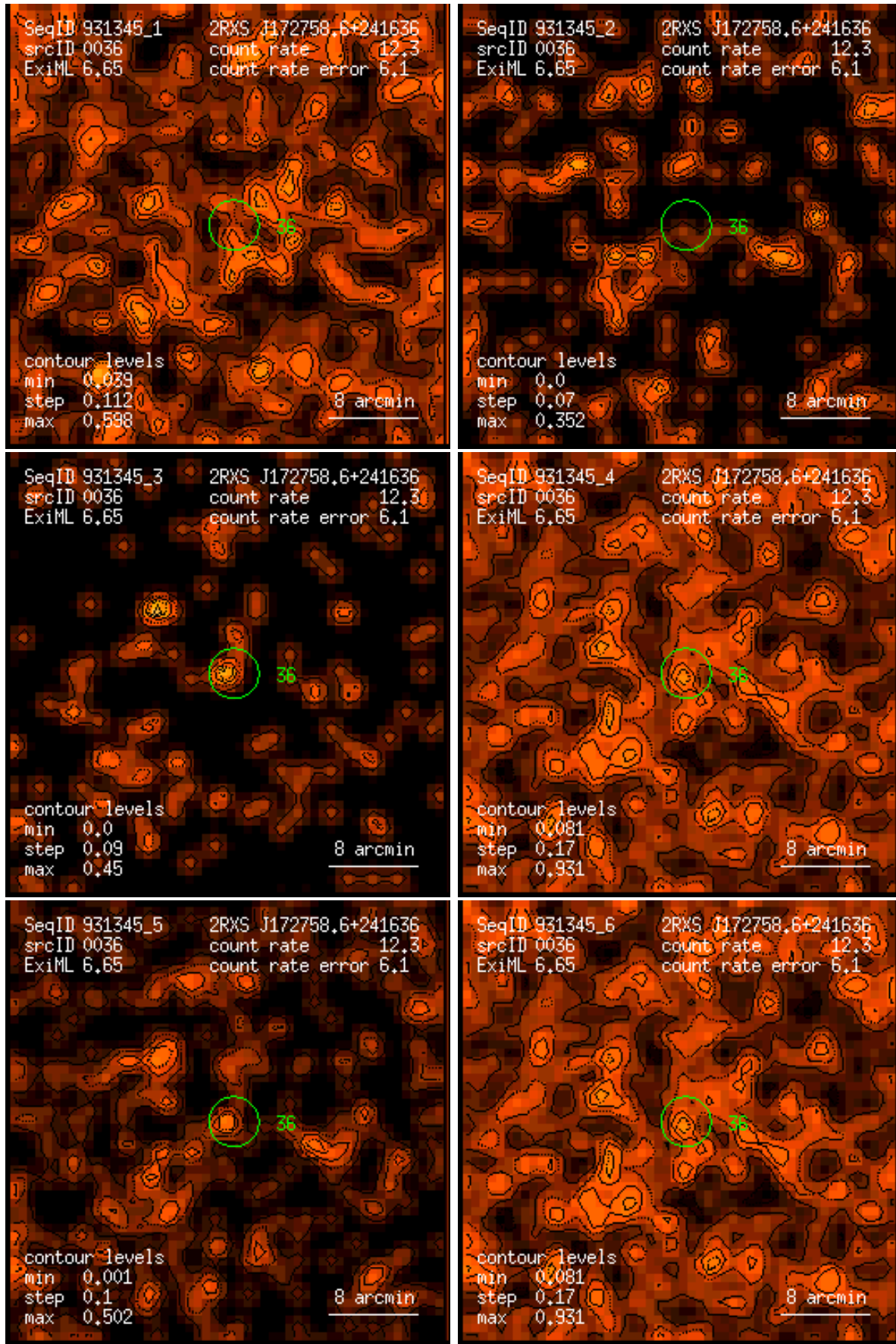
Figure 36: RASS 931345: detection 0036: band rate images, Gaussian filter: (1) PSPC channels 11 – 41, (2) 52 – 90, (3) 91 – 201, (4) 11 – 235, (5) 52 – 201, (6) 11 – 201. Broad band rates in counts/ks. Band rate contour levels in counts/ks/arcmin 2 .
