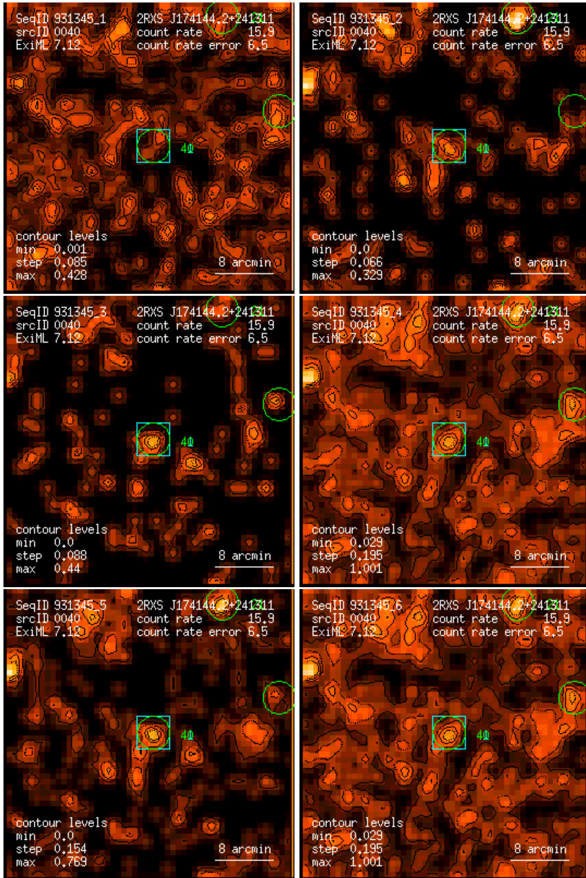
Figure 40: RASS 931345: detection 0040: band rate images, Gaussian filter: (1) PSPC channels 11 – 41, (2) 52 – 90, (3) 91 – 201, (4) 11 – 235, (5) 52 – 201, (6) 11 – 201. Broad band rates in counts/ks. Band rate contour levels in counts/ks/arcmin 2 .
