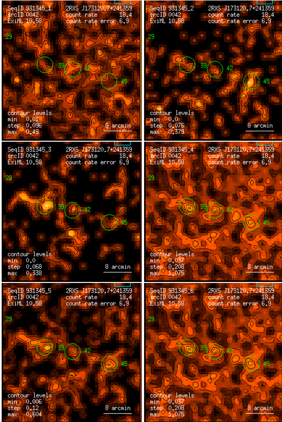
Figure 42: RASS 931345: detection 0042: band rate images, Gaussian filter: (1) PSPC channels 11 – 41, (2) 52 – 90, (3) 91 – 201, (4) 11 – 235, (5) 52 – 201, (6) 11 – 201. Broad band rates in counts/ks. Band rate contour levels in counts/ks/arcmin 2 .
