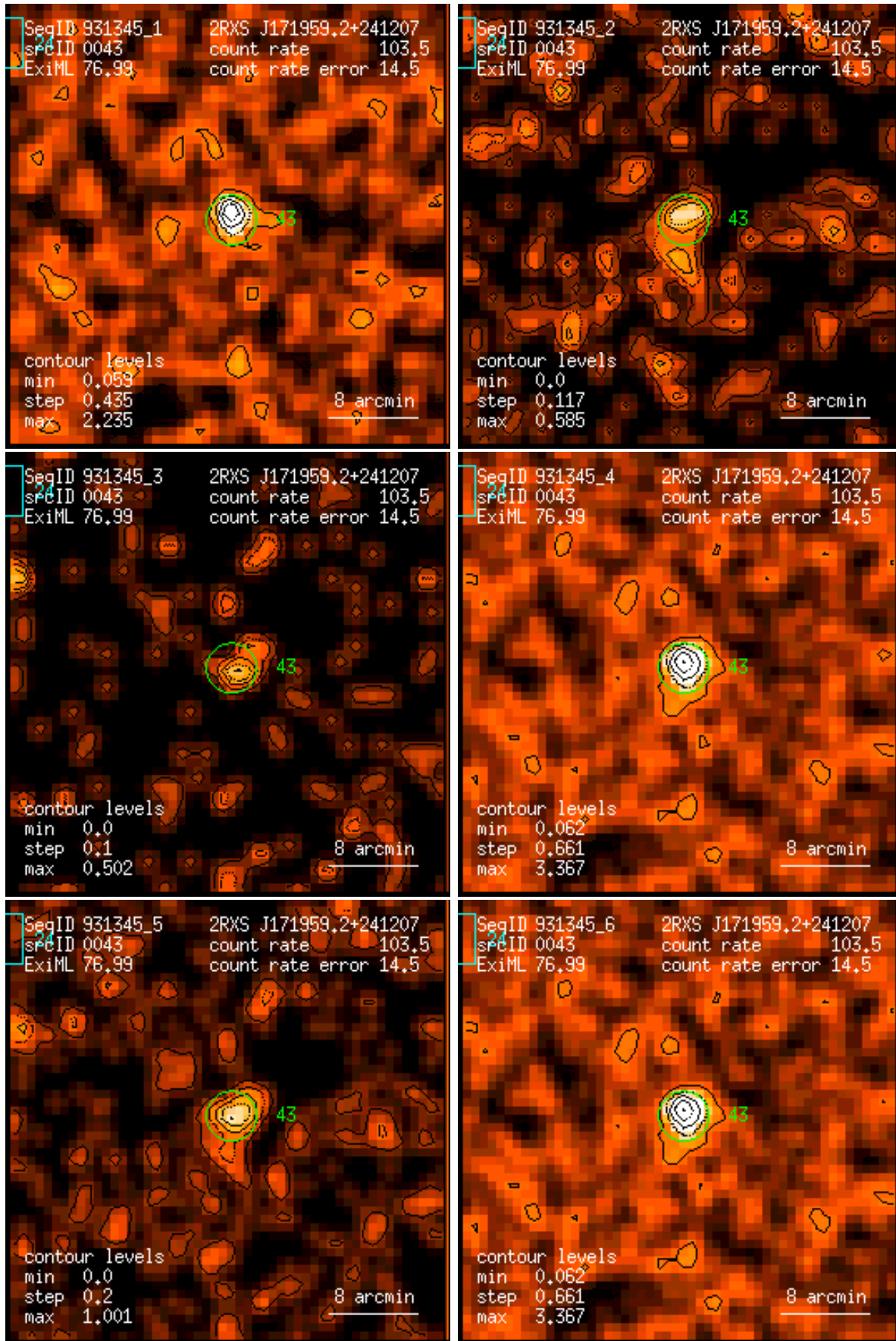
Figure 43: RASS 931345: detection 0043: band rate images, Gaussian filter: (1) PSPC channels 11 – 41, (2) 52 – 90, (3) 91 – 201, (4) 11 – 235, (5) 52 – 201, (6) 11 – 201. Broad band rates in counts/ks. Band rate contour levels in counts/ks/arcmin 2 .
