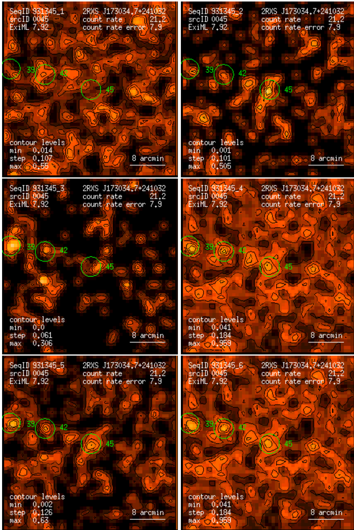
Figure 45: RASS 931345: detection 0045: band rate images, Gaussian filter: (1) PSPC channels 11 – 41, (2) 52 – 90, (3) 91 – 201, (4) 11 – 235, (5) 52 – 201, (6) 11 – 201. Broad band rates in counts/ks. Band rate contour levels in counts/ks/arcmin 2 .
