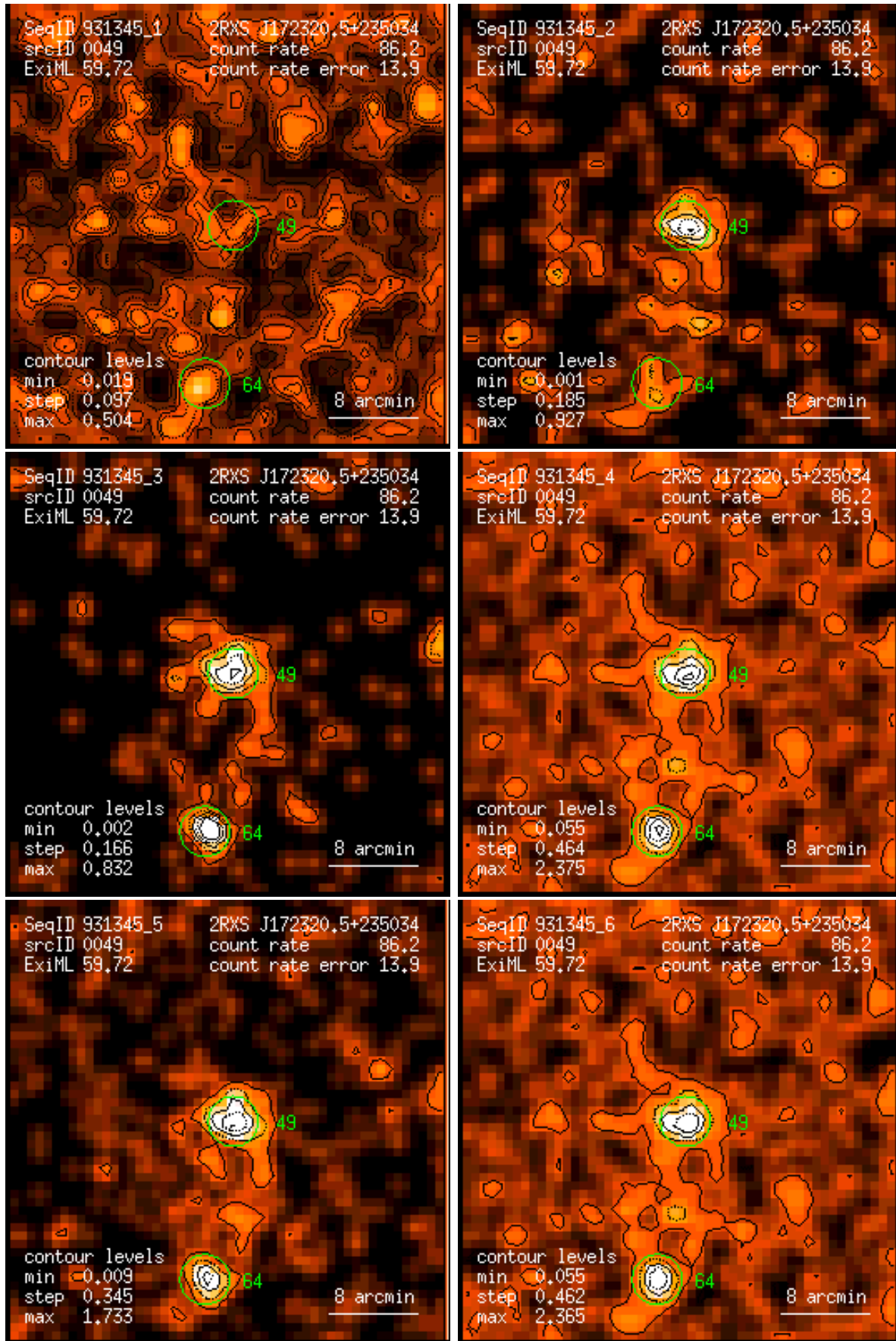
Figure 49: RASS 931345: detection 0049: band rate images, Gaussian filter: (1) PSPC channels 11 – 41, (2) 52 – 90, (3) 91 – 201, (4) 11 – 235, (5) 52 – 201, (6) 11 – 201. Broad band rates in counts/ks. Band rate contour levels in counts/ks/arcmin 2 .
