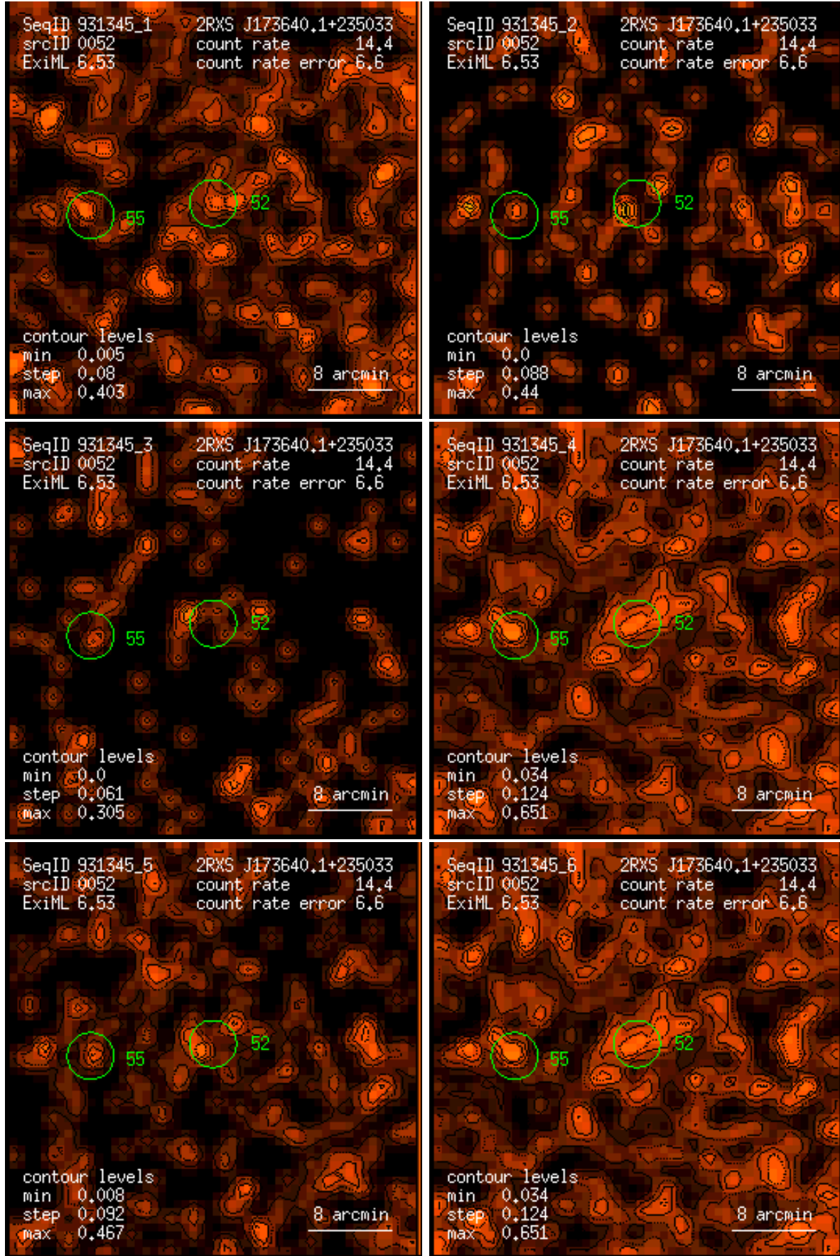
Figure 52: RASS 931345: detection 0052: band rate images, Gaussian filter: (1) PSPC channels 11 – 41, (2) 52 – 90, (3) 91 – 201, (4) 11 – 235, (5) 52 – 201, (6) 11 – 201. Broad band rates in counts/ks. Band rate contour levels in counts/ks/arcmin 2 .
