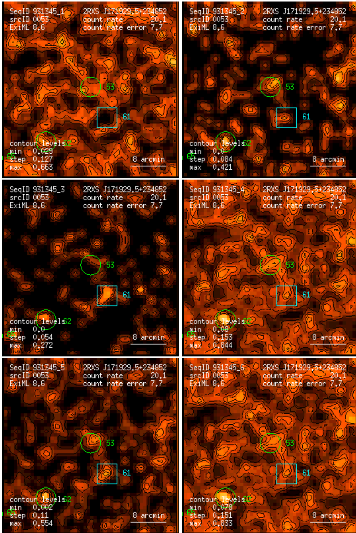
Figure 53: RASS 931345: detection 0053: band rate images, Gaussian filter: (1) PSPC channels 11 – 41, (2) 52 – 90, (3) 91 – 201, (4) 11 – 235, (5) 52 – 201, (6) 11 – 201. Broad band rates in counts/ks. Band rate contour levels in counts/ks/arcmin 2 .
