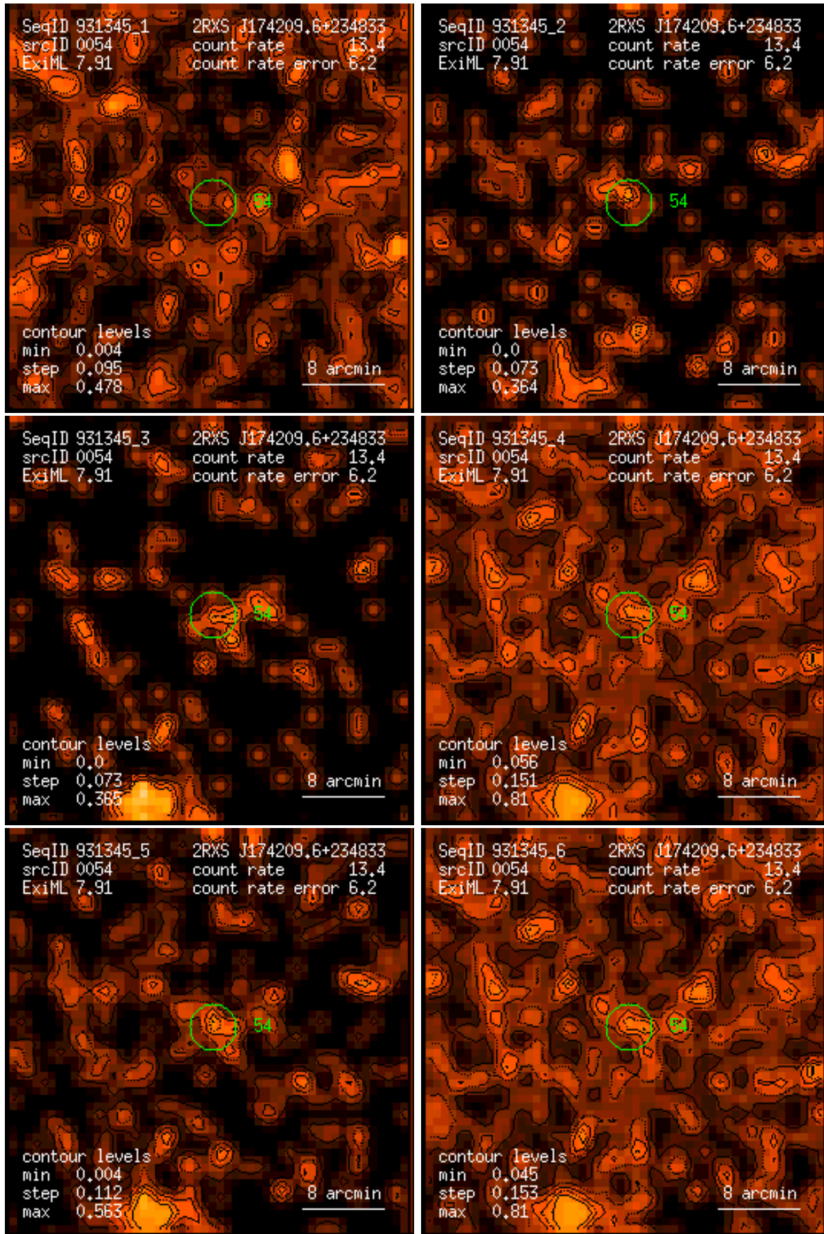
Figure 54: RASS 931345: detection 0054: band rate images, Gaussian filter: (1) PSPC channels 11 – 41, (2) 52 – 90, (3) 91 – 201, (4) 11 – 235, (5) 52 – 201, (6) 11 – 201. Broad band rates in counts/ks. Band rate contour levels in counts/ks/arcmin 2 .
