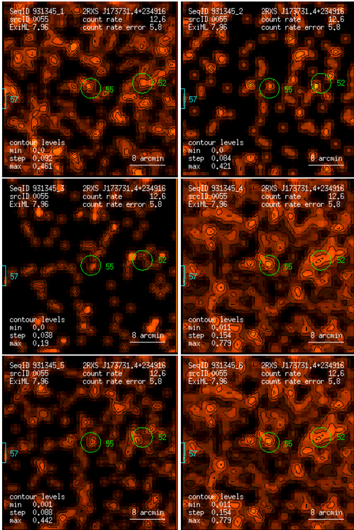
Figure 55: RASS 931345: detection 0055: band rate images, Gaussian filter: (1) PSPC channels 11 – 41, (2) 52 – 90, (3) 91 – 201, (4) 11 – 235, (5) 52 – 201, (6) 11 – 201. Broad band rates in counts/ks. Band rate contour levels in counts/ks/arcmin 2 .
