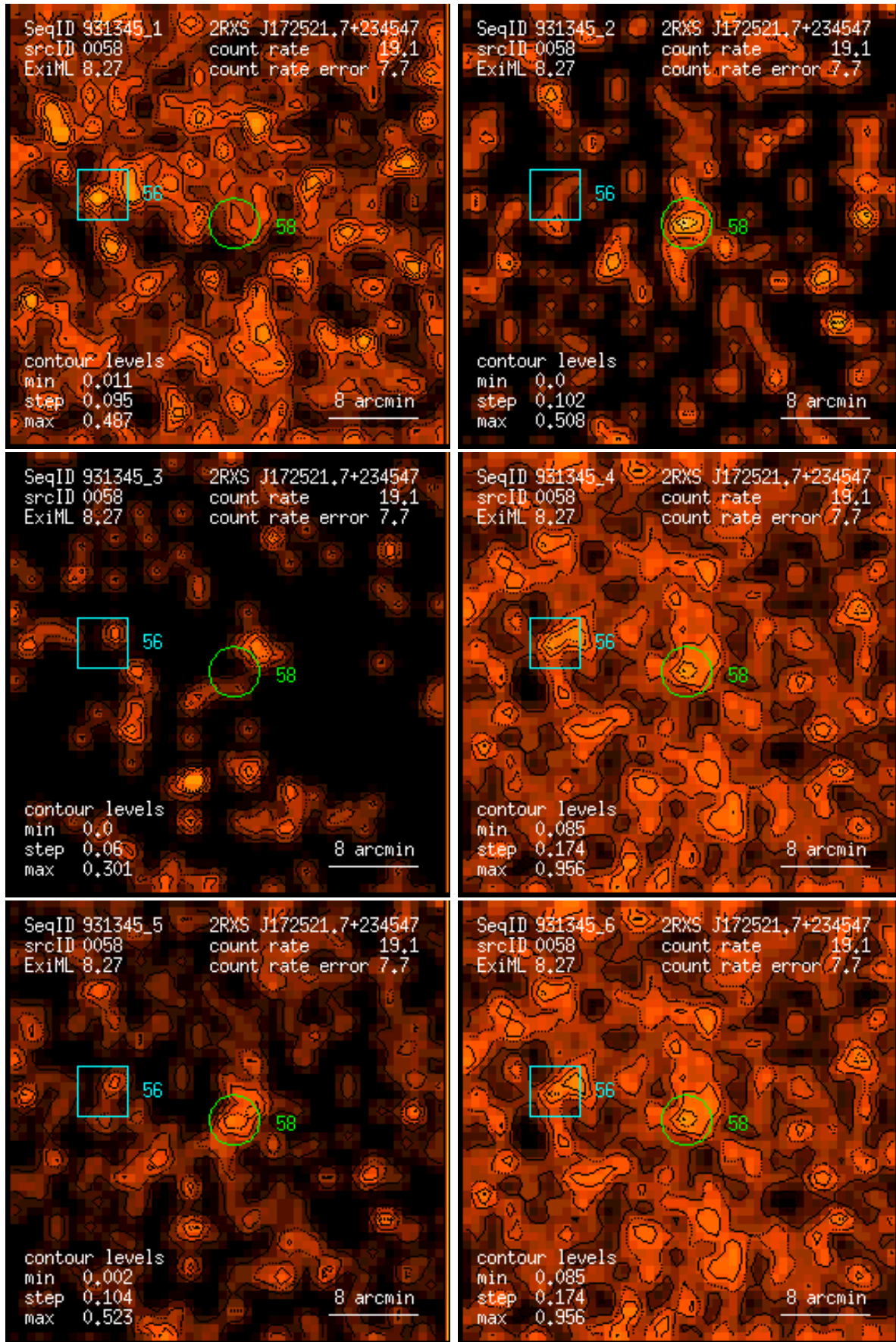
Figure 58: RASS 931345: detection 0058: band rate images, Gaussian filter: (1) PSPC channels 11 – 41, (2) 52 – 90, (3) 91 – 201, (4) 11 – 235, (5) 52 – 201, (6) 11 – 201. Broad band rates in counts/ks. Band rate contour levels in counts/ks/arcmin 2 .
