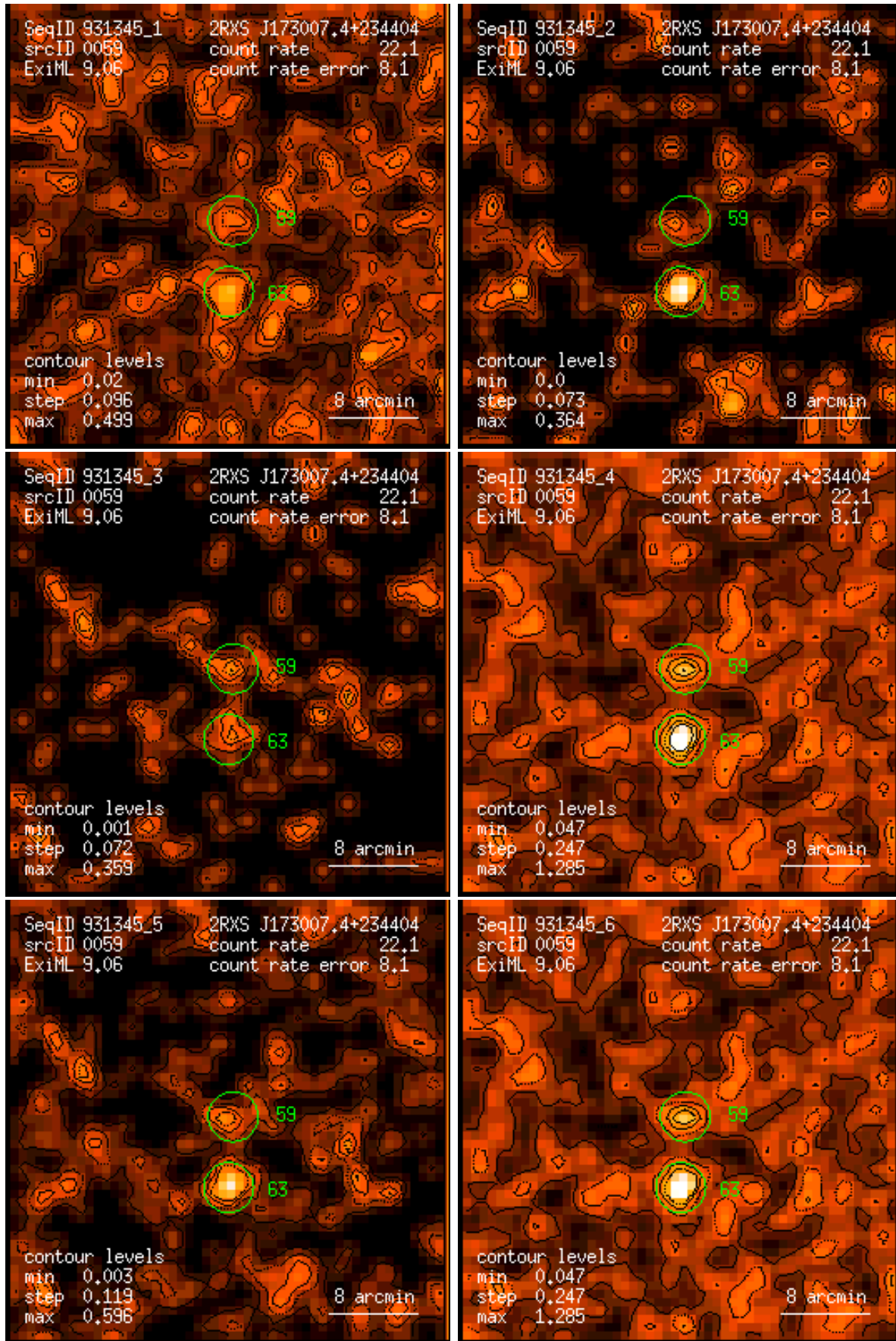
Figure 59: RASS 931345: detection 0059: band rate images, Gaussian filter: (1) PSPC channels 11 – 41, (2) 52 – 90, (3) 91 – 201, (4) 11 – 235, (5) 52 – 201, (6) 11 – 201. Broad band rates in counts/ks. Band rate contour levels in counts/ks/arcmin 2 .
