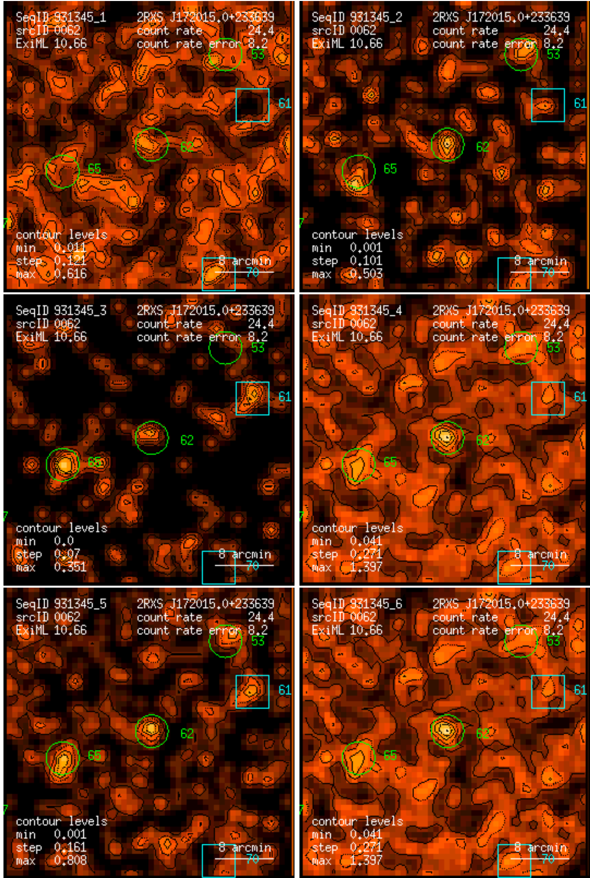
Figure 62: RASS 931345: detection 0062: band rate images, Gaussian filter: (1) PSPC channels 11 – 41, (2) 52 – 90, (3) 91 – 201, (4) 11 – 235, (5) 52 – 201, (6) 11 – 201. Broad band rates in counts/ks. Band rate contour levels in counts/ks/arcmin 2 .
