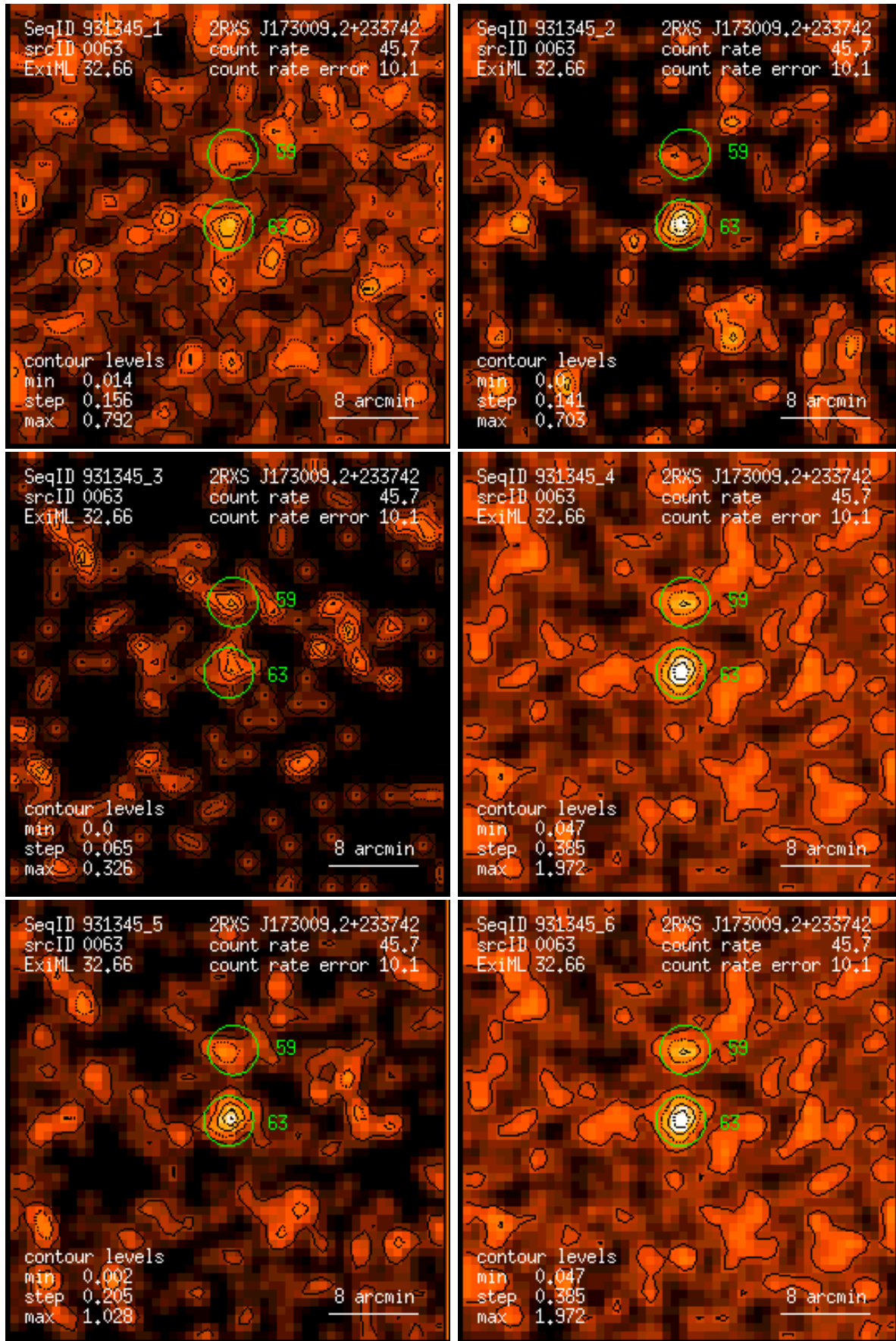
Figure 63: RASS 931345: detection 0063: band rate images, Gaussian filter: (1) PSPC channels 11 – 41, (2) 52 – 90, (3) 91 – 201, (4) 11 – 235, (5) 52 – 201, (6) 11 – 201. Broad band rates in counts/ks. Band rate contour levels in counts/ks/arcmin 2 .
